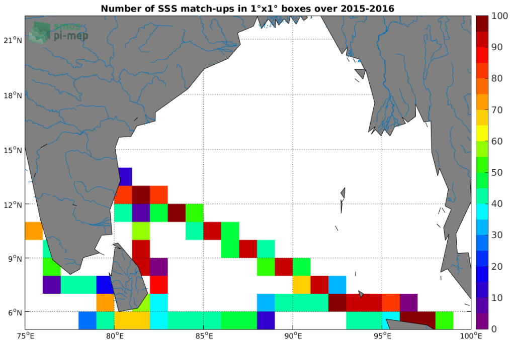
Figure 4: Number of SSS match-ups between TSG-LEGOS-DM SSS and the SMAP-L3-JPL-V4.3-MONTHLY-60KM SSS product for the Ganga and Brahmaputra river plumes Pi-MEP region over 1^\circ \times 1^\circ boxes and for the full satellite product period.
