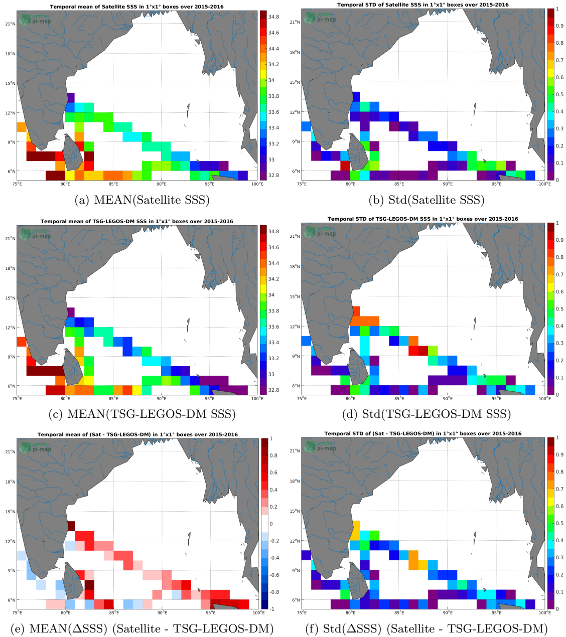
Figure 6: Temporal mean (left) and Std (right) of SSS from SMAP-L3-JPL-V4.3-MONTHLY-60KM (top), TSG-LEGOS-DM (middle), and of \Delta SSS (Satellite - TSG-LEGOS-DM). Only match-up pairs are used to generate these maps.
