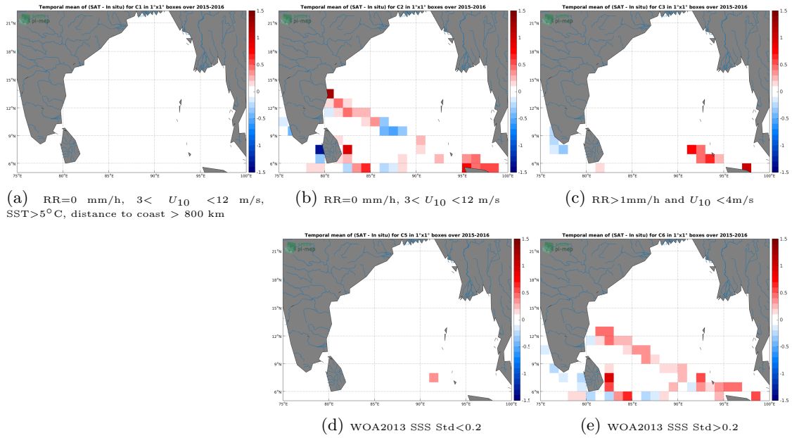
Figure 12: Temporal mean gridded over spatial boxes of size 1^\circ \times 1^\circ of \Delta SSS (SMAP-L3-JPL-V4.3-MONTHLY-60KM - TSG-LEGOS-DM) for 5 different subdatasets corresponding to:RR=0 mm/h, 3 < U_{10} < 12 m/s, SST >5^\circ C, distance to coast > 800 km (a), RR=0 mm/h, 3 < U_{10} < 12 m/s (b), RR >1 mm/h and U_{10} < 4 m/s (c), WOA2013 SSS Std <0.2 (d), WOA2013 SSS Std >0.2 (e).
