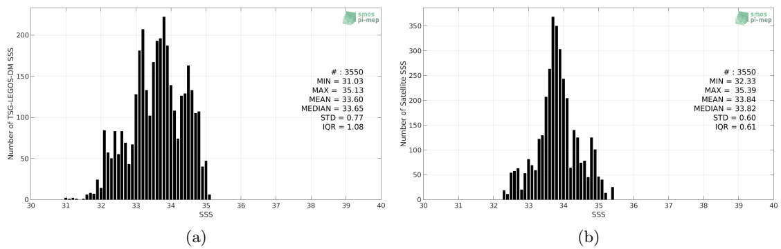
Figure 2: Histograms of SSS from TSG-LEGOS-DM (a) and SMAP-L3-JPL-V4.3-MONTHLY-60KM (b) considering all match-up pairs per bins of 0.1 over the Ganga and Brahmaputra river plumes Pi-MEP region and for the full satellite product period.
