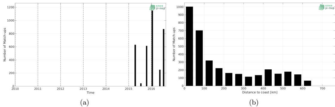
Figure 1: Number of match-ups between TSG-LEGOS-DM and SMAP-L3-JPL-V4.3-MONTHLY-60KM SSS as a function of time (a) and as function of the distance to coast (b) over the Ganga and Brahmaputra river plumes Pi-MEP region and for the full satellite product period.
