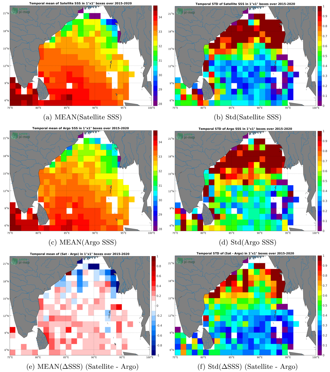
Figure 6: Temporal mean (left) and Std (right) of SSS from SMAP-L3-JPL-V4.3-MONTHLY-60KM (top), Argo (middle), and of \Delta SSS (Satellite - Argo). Only match-up pairs are used to generate these maps.
