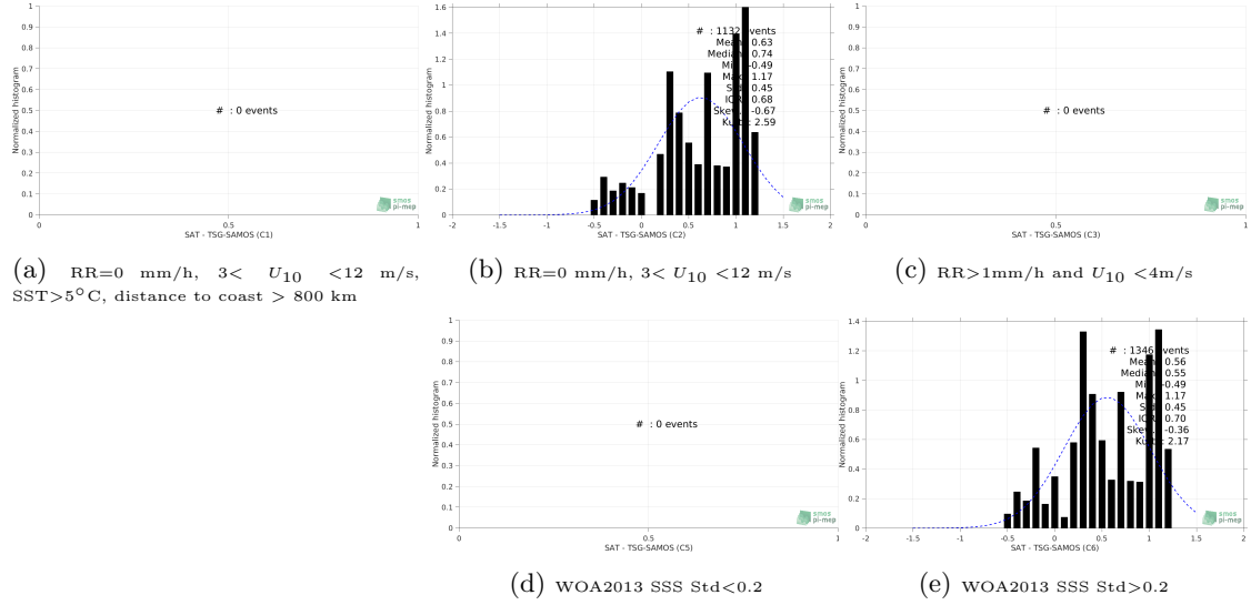
Figure 13: Normalized histogram of \Delta SSS (SMAP-L3-JPL-V4.2-8DAY-RUNNING-60KM - TSG-SAMOS) for 5 different subdatasets corresponding to: RR=0 mm/h, 3 < U_{10} < 12 m/s, SST>5°C, distance to coast > 800 km (a), RR=0 mm/h, 3 < U_{10} < 12 m/s (b), RR>1mm/h and U_{10} < 4 m/s (c), WOA2013 SSS Std<0.2 (d), WOA2013 SSS Std>0.2 (e).
