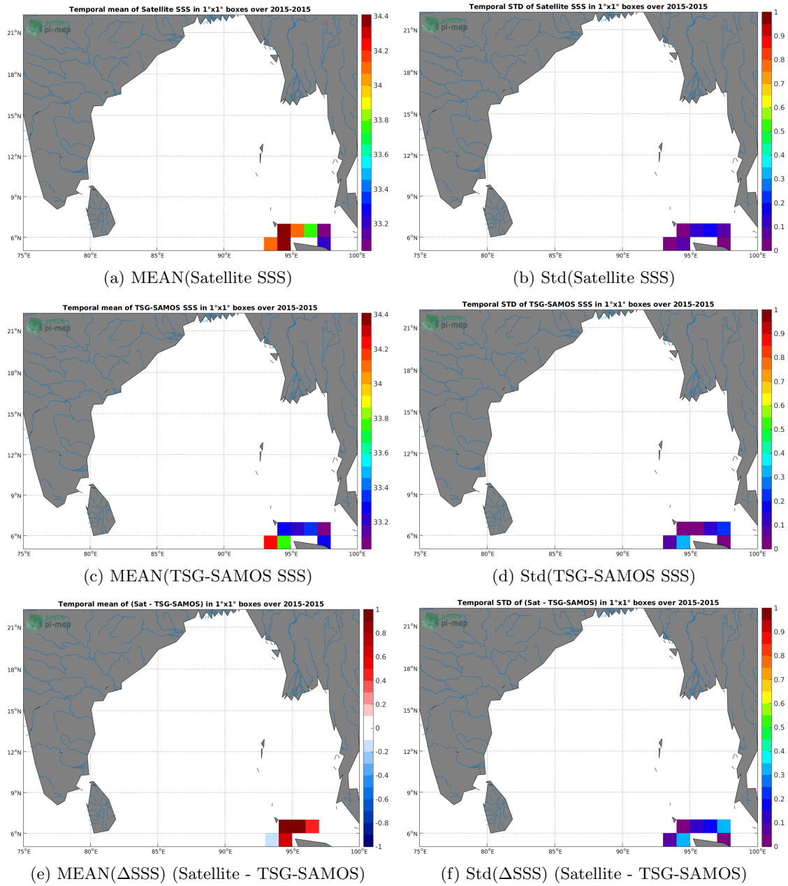
Figure 6: Temporal mean (left) and Std (right) of SSS from SMAP-L3-JPL-V4.2-8DAY-RUNNING-60KM (top), TSG-SAMOS (middle), and of \Delta SSS (Satellite - TSG-SAMOS). Only match-up pairs are used to generate these maps.
