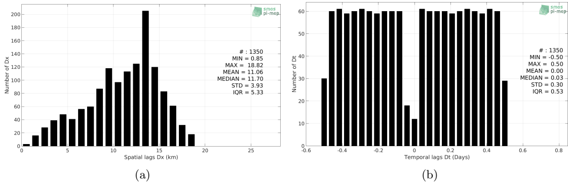
Figure 5: Histograms of the spatial (a) and temporal (b) lags between the time of the TSG-SAMOS measurements and the date of the corresponding SMAP-L3-JPL-V4.2-8DAY-RUNNING-60KM SSS product.
