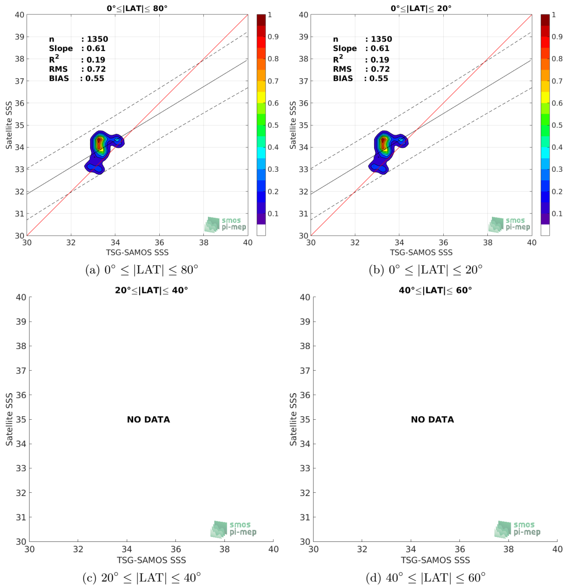
Figure 9: Contour maps of the concentration of SMAP-L3-JPL-V4.2-8DAY-RUNNING-60KM SSS (y-axis) versus TSG-SAMOS SSS (x-axis) at match-up pairs for different latitude bands. For each plot, the red line shows x=y . The black thin and dashed lines indicate a linear fit through the data cloud and the \pm 95\% confidence levels, respectively. The number match-up pairs n , the slope and R^2 coefficient of the linear fit, the root mean square (RMS) and the mean bias between satellite and in situ data are indicated for each latitude band in each plots.
