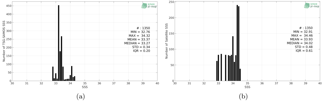
Figure 2: Histograms of SSS from TSG-SAMOS (a) and SMAP-L3-JPL-V4.2-8DAY-RUNNING-60KM (b) considering all match-up pairs per bins of 0.1 over the Ganga and Brahmaputra river plumes Pi-MEP region and for the full satellite product period.
