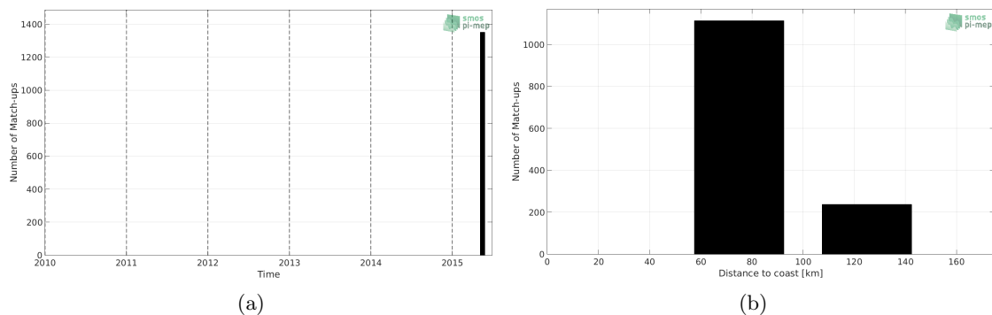
Figure 1: Number of match-ups between TSG-SAMOS and SMAP-L3-JPL-V4.2-8DAY-RUNNING-60KM SSS as a function of time (a) and as function of the distance to coast (b) over the Ganga and Brahmaputra river plumes Pi-MEP region and for the full satellite product period.
