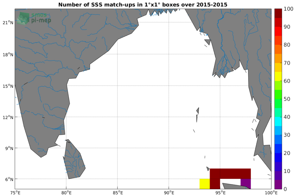
Figure 4: Number of SSS match-ups between TSG-SAMOS SSS and the SMAP-L3-JPL-V4.2-8DAY-RUNNING-60KM SSS product for the Ganga and Brahmaputra river plumes Pi-MEP region over 1°x1° boxes and for the full satellite product period.
