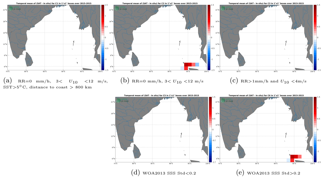
Figure 12: Temporal mean gridded over spatial boxes of size 1^\circ \times 1^\circ of \Delta SSS (SMAP-L3-JPL-V4.2-8DAY-RUNNING-60KM - TSG-SAMOS) for 5 different subdatasets corresponding to:RR=0 mm/h, 3 < U_{10} < 12 m/s, SST > 5^\circ\text{C} , distance to coast > 800 km (a), RR=0 mm/h, 3 < U_{10} < 12 m/s (b), RR > 1 mm/h and U_{10} < 4 m/s (c), WOA2013 SSS Std < 0.2 (d), WOA2013 SSS Std > 0.2 (e).
