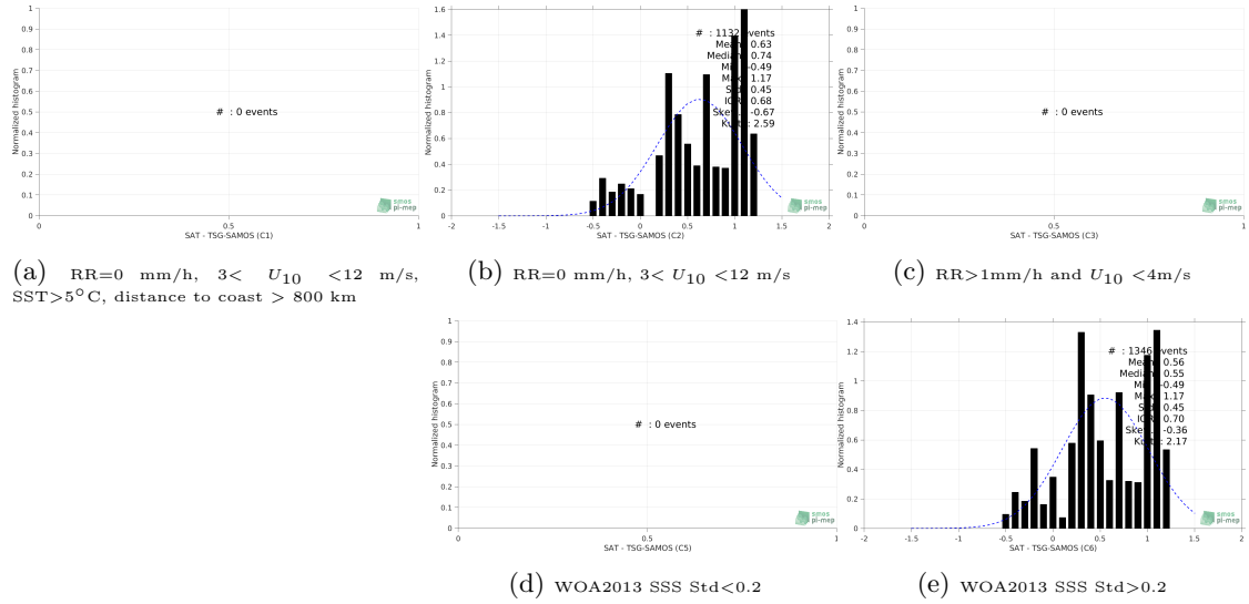
Figure 13: Normalized histogram of \Delta\text{SSS} (SMAP-L3-JPL-V4.2-8DAY-RUNNING-60KM - TSG-SAMOS) for 5 different subdatasets corresponding to: RR=0 mm/h, 3 < U_{10} < 12 m/s, SST > 5^\circ\text{C} , distance to coast > 800 km (a), RR=0 mm/h, 3 < U_{10} < 12 m/s (b), RR > 1\text{mm/h} and U_{10} < 4\text{m/s} (c), WOA2013 SSS Std < 0.2 (d), WOA2013 SSS Std > 0.2 (e).
