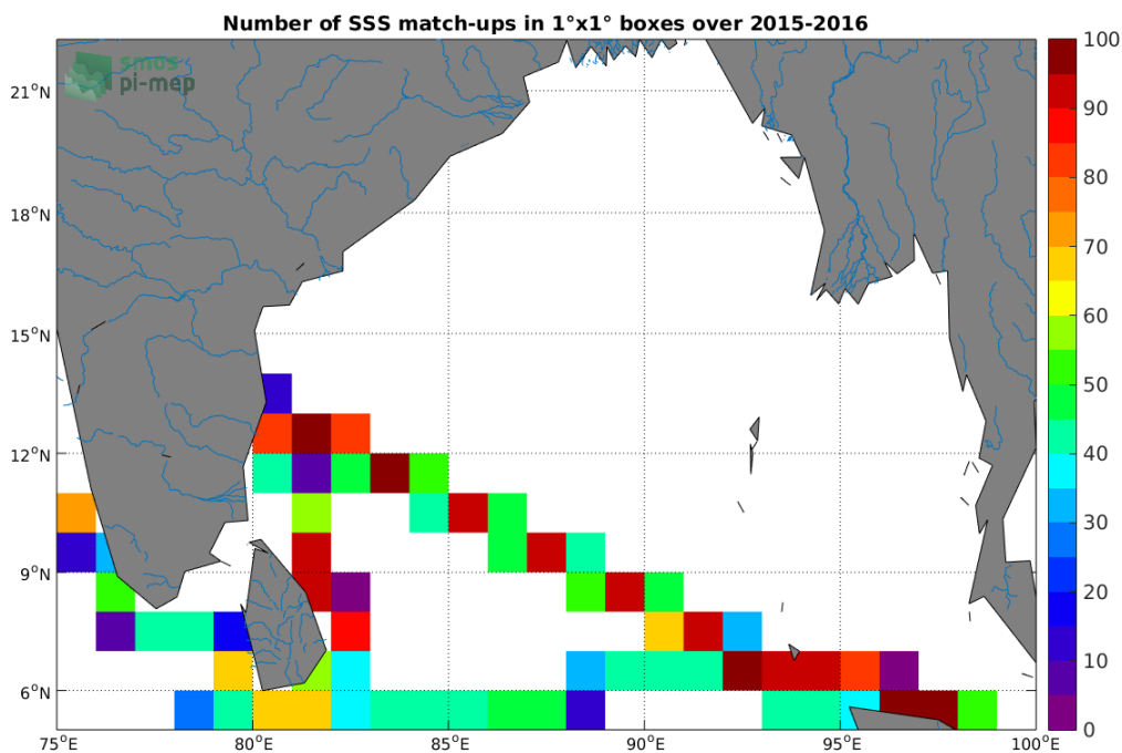
Figure 4: Number of SSS match-ups between TSG-LEGOS-DM SSS and the SMAP-L3-JPL-V4.2-8DAY-RUNNING-60KM SSS product for the Ganga and Brahmaputra river plumes Pi-MEP region over 1^\circ \times 1^\circ boxes and for the full satellite product period.
