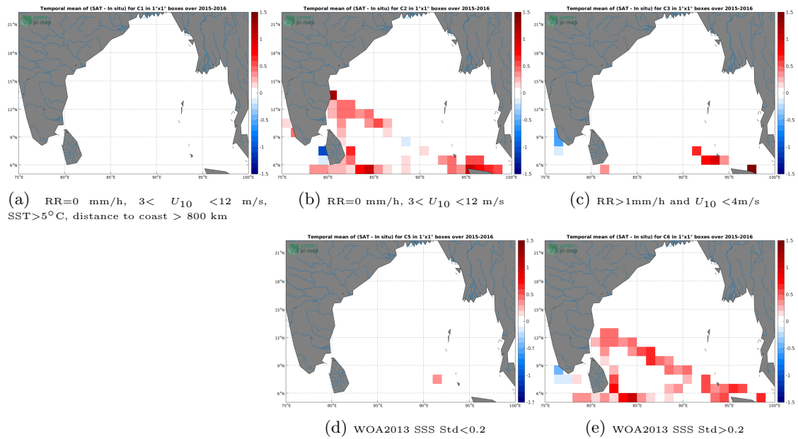
Figure 12: Temporal mean gridded over spatial boxes of size 1^\circ \times 1^\circ of \Delta SSS (SMAP-L3-JPL-V4.2-8DAY-RUNNING-60KM - TSG-LEGOS-DM) for 5 different subdatasets corresponding to:RR=0 mm/h, 3 < U_{10} < 12 m/s, SST > 5^\circ\text{C} , distance to coast > 800 km (a), RR=0 mm/h, 3 < U_{10} < 12 m/s (b), RR > 1 mm/h and U_{10} < 4 m/s (c), WOA2013 SSS Std < 0.2 (d), WOA2013 SSS Std > 0.2 (e).
