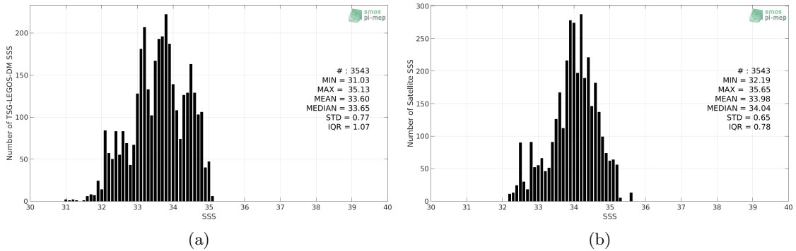
Figure 2: Histograms of SSS from TSG-LEGOS-DM (a) and SMAP-L3-JPL-V4.2-8DAY-RUNNING-60KM (b) considering all match-up pairs per bins of 0.1 over the Ganga and Brahmaputra river plumes Pi-MEP region and for the full satellite product period.
