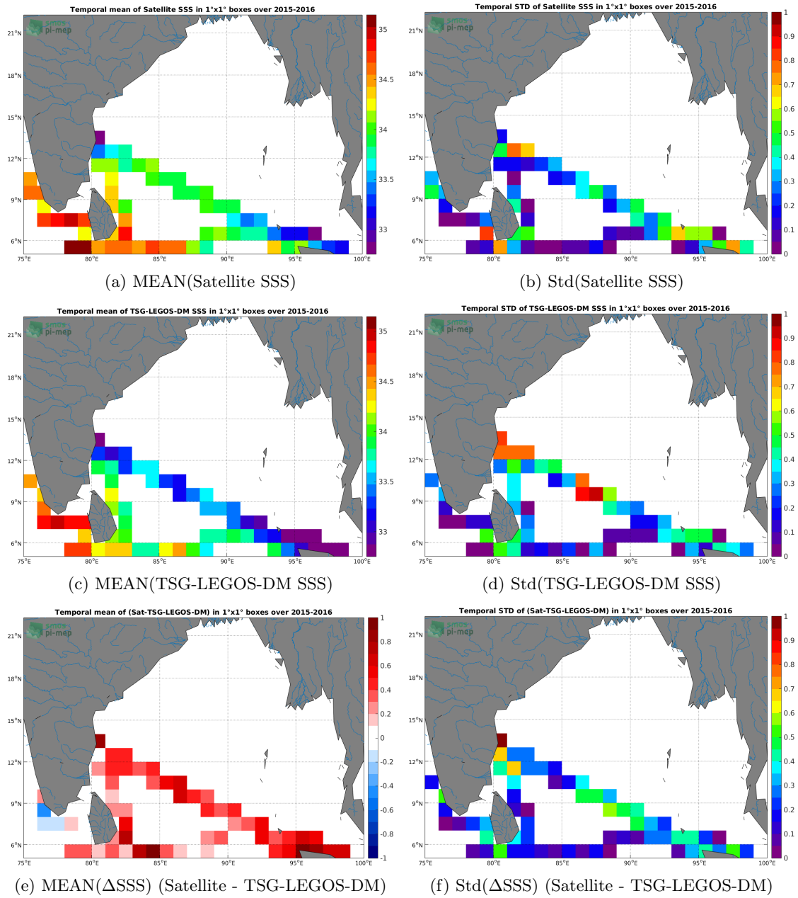
Figure 6: Temporal mean (left) and Std (right) of SSS from SMAP-L3-JPL-V4.2-8DAY-RUNNING-60KM (top), TSG-LEGOS-DM (middle), and of \Delta SSS (Satellite - TSG-LEGOS-DM). Only match-up pairs are used to generate these maps.
