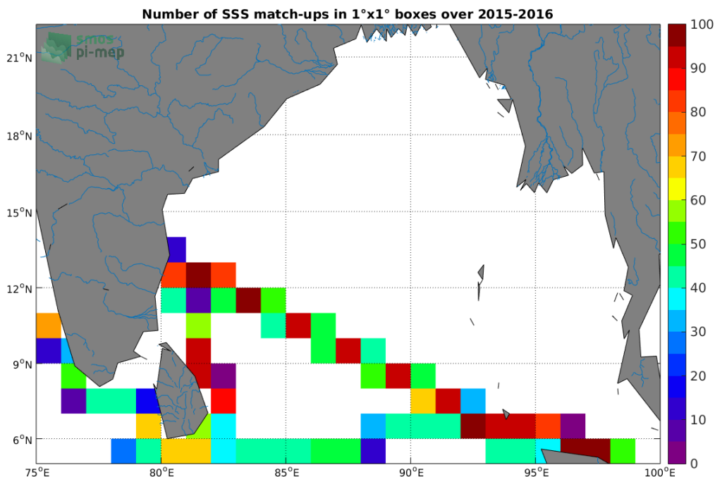
Figure 4: Number of SSS match-ups between TSG-LEGOS-DM SSS and the SMAP-L3-JPL-V4.2-8DAY-RUNNING-60KM SSS product for the Ganga and Brahmaputra river plumes Pi-MEP region over 1°x1° boxes and for the full satellite product period.
