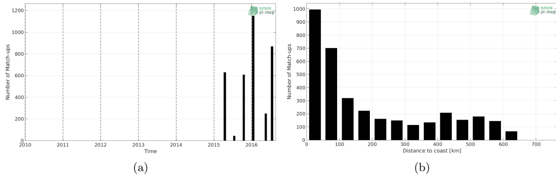
Figure 1: Number of match-ups between TSG-LEGOS-DM and SMAP-L3-JPL-V4.2-8DAY-RUNNING-60KM SSS as a function of time (a) and as function of the distance to coast (b) over the Ganga and Brahmaputra river plumes Pi-MEP region and for the full satellite product period.
