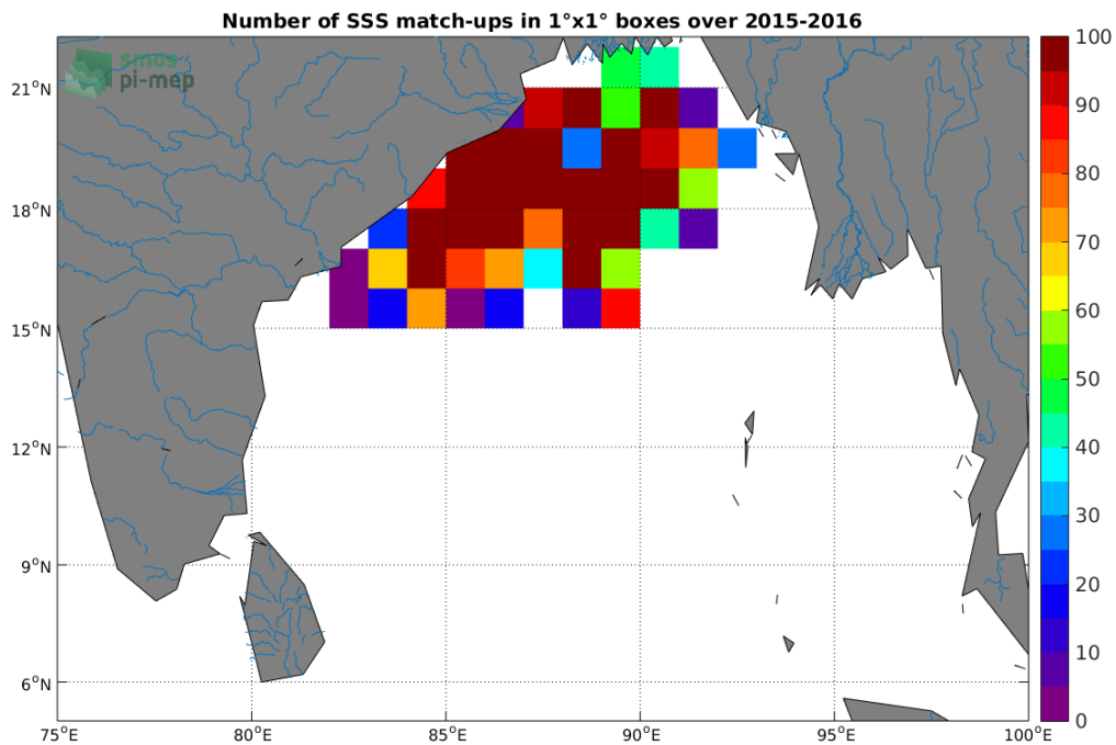
Figure 3: Number of SSS match-ups between Surface drifters SSS and the SMAP-L3-JPL-V4.2-8DAY-RUNNING-60KM SSS product for the Ganga and Brahmaputra river plumes Pi-MEP region over 1°x1° boxes and for the full satellite product period.
