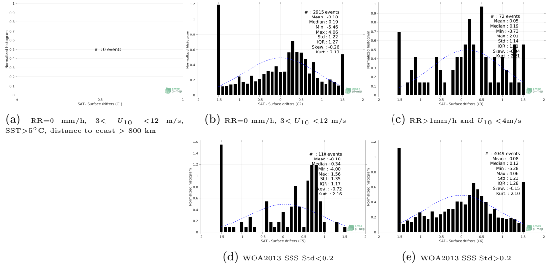
Figure 12: Normalized histogram of \Delta SSS (SMAP-L3-JPL-V4.2-8DAY-RUNNING-60KM - Surface drifters) for 5 different subdatasets corresponding to: RR=0 mm/h, 3 < U_{10} < 12 m/s, SST > 5°C, distance to coast > 800 km (a), RR=0 mm/h, 3 < U_{10} < 12 m/s (b), RR > 1mm/h and U_{10} < 4 m/s (c), WOA2013 SSS Std < 0.2 (d), WOA2013 SSS Std > 0.2 (e).
