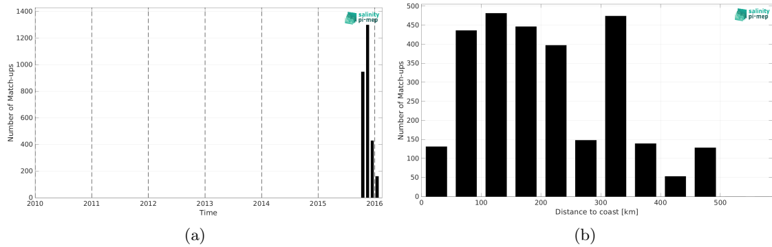
Figure 2: Number of match-ups between Surface drifters and SMAP SSS L2 v6 - 40 km (RSS) SSS as a function of time (a) and as function of the distance to coast (b) over the Ganga and Brahmaputra river plumes Pi-MEP region and for the full satellite product period.
