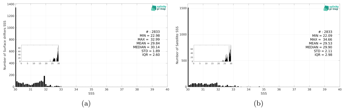
Figure 3: Histograms of SSS from Surface drifters (a) and SMAP SSS L2 v6 - 40 km (RSS) (b) considering all match-up pairs per bins of 0.1 over the Ganga and Brahmaputra river plumes Pi-MEP region and for the full satellite product period.
