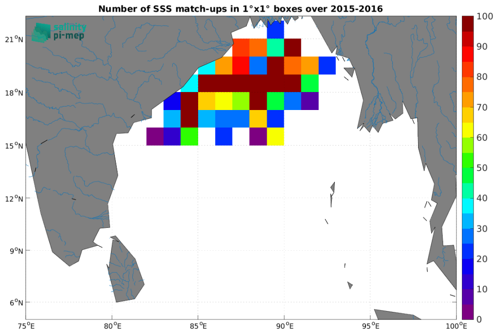
Figure 4: Number of SSS match-ups between Surface drifters SSS and the SMAP SSS L2 v6 - 40 km (RSS) SSS product for the Ganga and Brahmaputra river plumes Pi-MEP region over 1^\circ \times 1^\circ boxes and for the full satellite product period.
