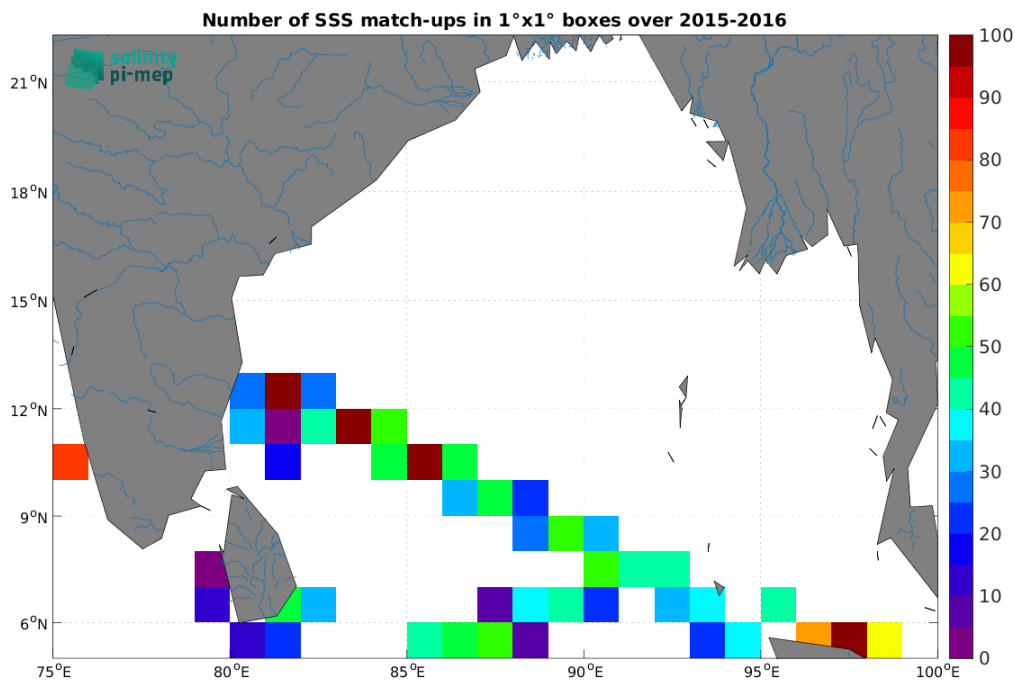
Figure 4: Number of SSS match-ups between TSG (LEGOS-DM) SSS and the SMAP SSS L2 v5 (RSS) SSS product for the Ganga and Brahmaputra river plumes Pi-MEP region over 1°×1° boxes and for the full satellite product period.
