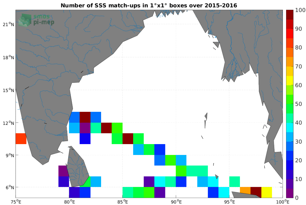
Figure 4: Number of SSS match-ups between TSG (LEGOS-DM) SSS and the SMAP SSS L2 v5 (RSS) SSS product for the Ganga and Brahmaputra river plumes Pi-MEP region over 1°x1° boxes and for the full satellite product period.
