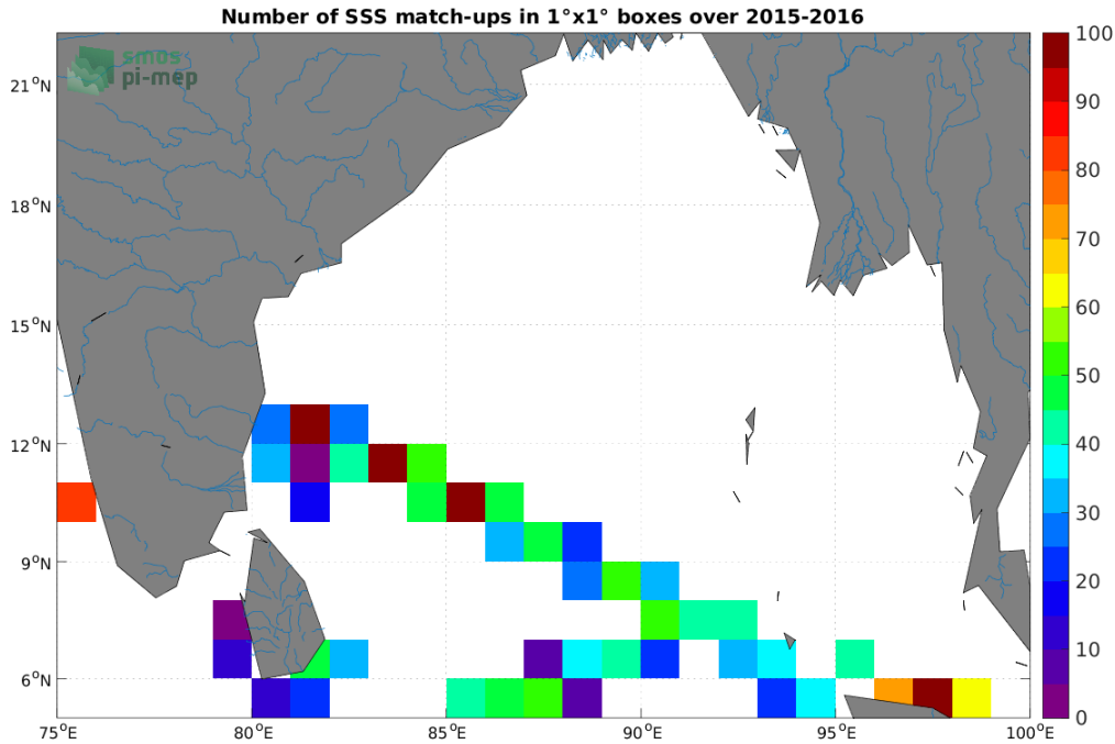
Figure 4: Number of SSS match-ups between TSG (LEGOS-DM) SSS and the SMAP SSS L2 v5 (RSS) SSS product for the Ganga and Brahmaputra river plumes Pi-MEP region over 1^\circ \times 1^\circ boxes and for the full satellite product period.
