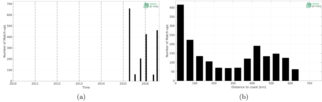
Figure 1: Number of match-ups between TSG (LEGOS-DM) and SMAP SSS L2 v5 (RSS) SSS as a function of time (a) and as function of the distance to coast (b) over the Ganga and Brahmaputra river plumes Pi-MEP region and for the full satellite product period.
