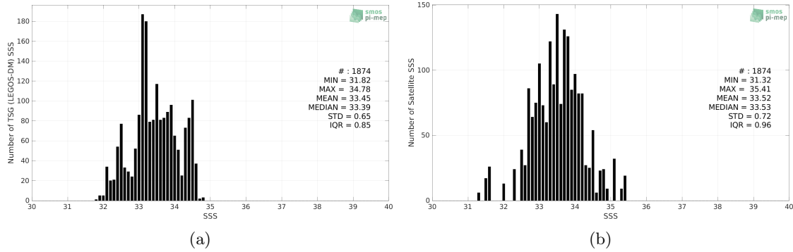
Figure 2: Histograms of SSS from TSG (LEGOS-DM) (a) and SMAP SSS L2 v5 (RSS) (b) considering all match-up pairs per bins of 0.1 over the Ganga and Brahmaputra river plumes Pi-MEP region and for the full satellite product period.
