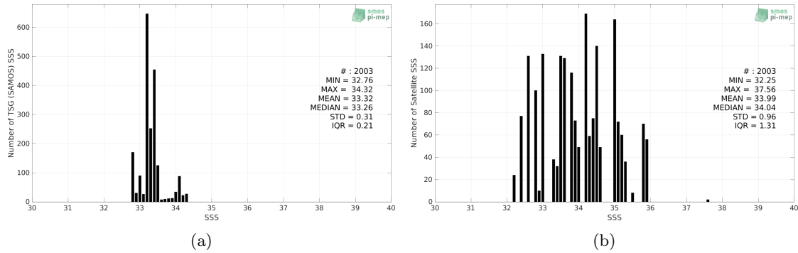
Figure 2: Histograms of SSS from TSG (SAMOS) (a) and SMAP SSS L2 v5 - 40 km (RSS) (b) considering all match-up pairs per bins of 0.1 over the Ganga and Brahmaputra river plumes Pi-MEP region and for the full satellite product period.
