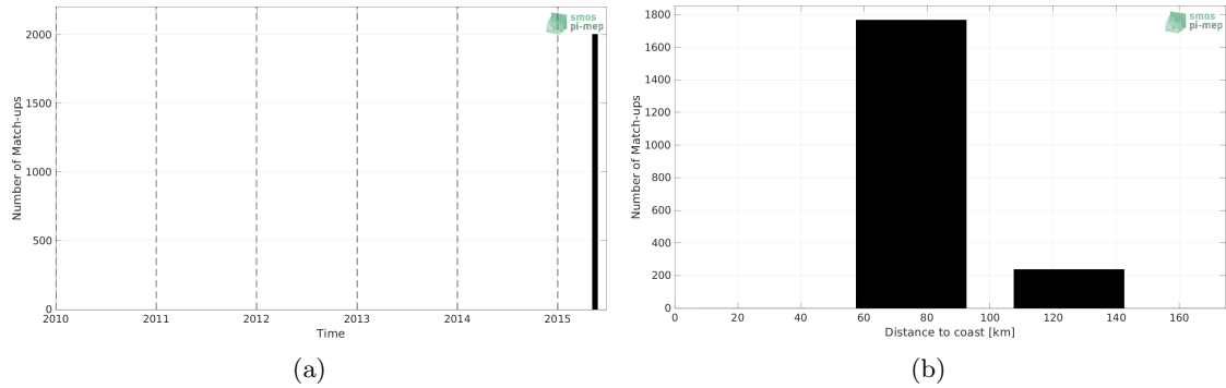
Figure 1: Number of match-ups between TSG (SAMOS) and SMAP SSS L2 v5 - 40 km (RSS) SSS as a function of time (a) and as function of the distance to coast (b) over the Ganga and Brahmaputra river plumes Pi-MEP region and for the full satellite product period.
