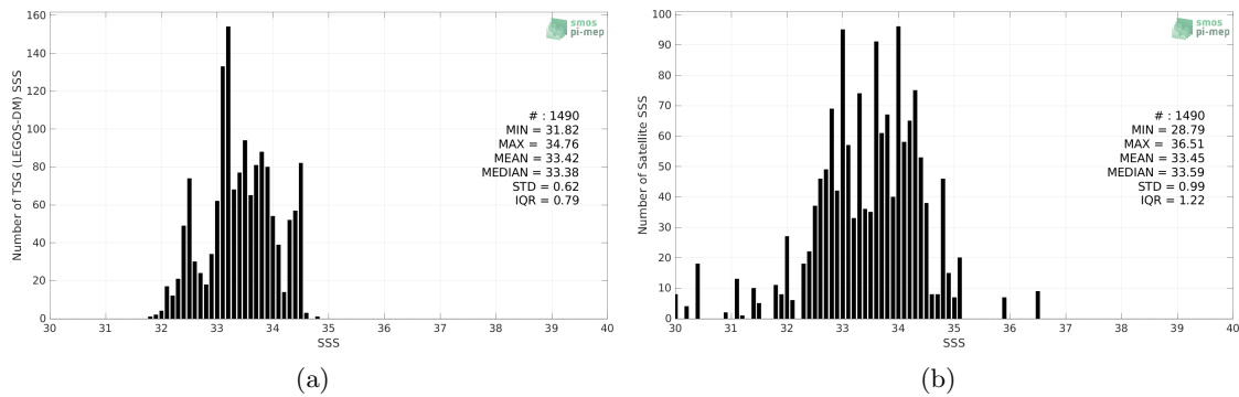
Figure 2: Histograms of SSS from TSG (LEGOS-DM) (a) and SMAP SSS L2 v5 - 40 km (RSS) (b) considering all match-up pairs per bins of 0.1 over the Ganga and Brahmaputra river plumes Pi-MEP region and for the full satellite product period.
