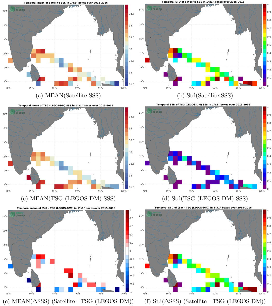
Figure 6: Temporal mean (left) and Std (right) of SSS from SMAP SSS L2 v5 - 40 km (RSS) (top), TSG (LEGOS-DM) (middle), and of \Delta SSS (Satellite - TSG (LEGOS-DM)). Only match-pairs are used to generate these maps.
