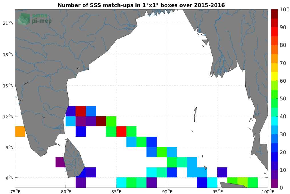
Figure 4: Number of SSS match-ups between TSG (LEGOS-DM) SSS and the SMAP SSS L2 v5 - 40 km (RSS) SSS product for the Ganga and Brahmaputra river plumes Pi-MEP region over 1^\circ \times 1^\circ boxes and for the full satellite product period.
