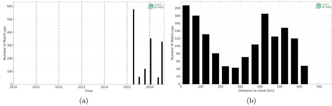
Figure 1: Number of match-ups between TSG (LEGOS-DM) and SMAP SSS L2 v5 - 40 km (RSS) SSS as a function of time (a) and as function of the distance to coast (b) over the Ganga and Brahmaputra river plumes Pi-MEP region and for the full satellite product period.
