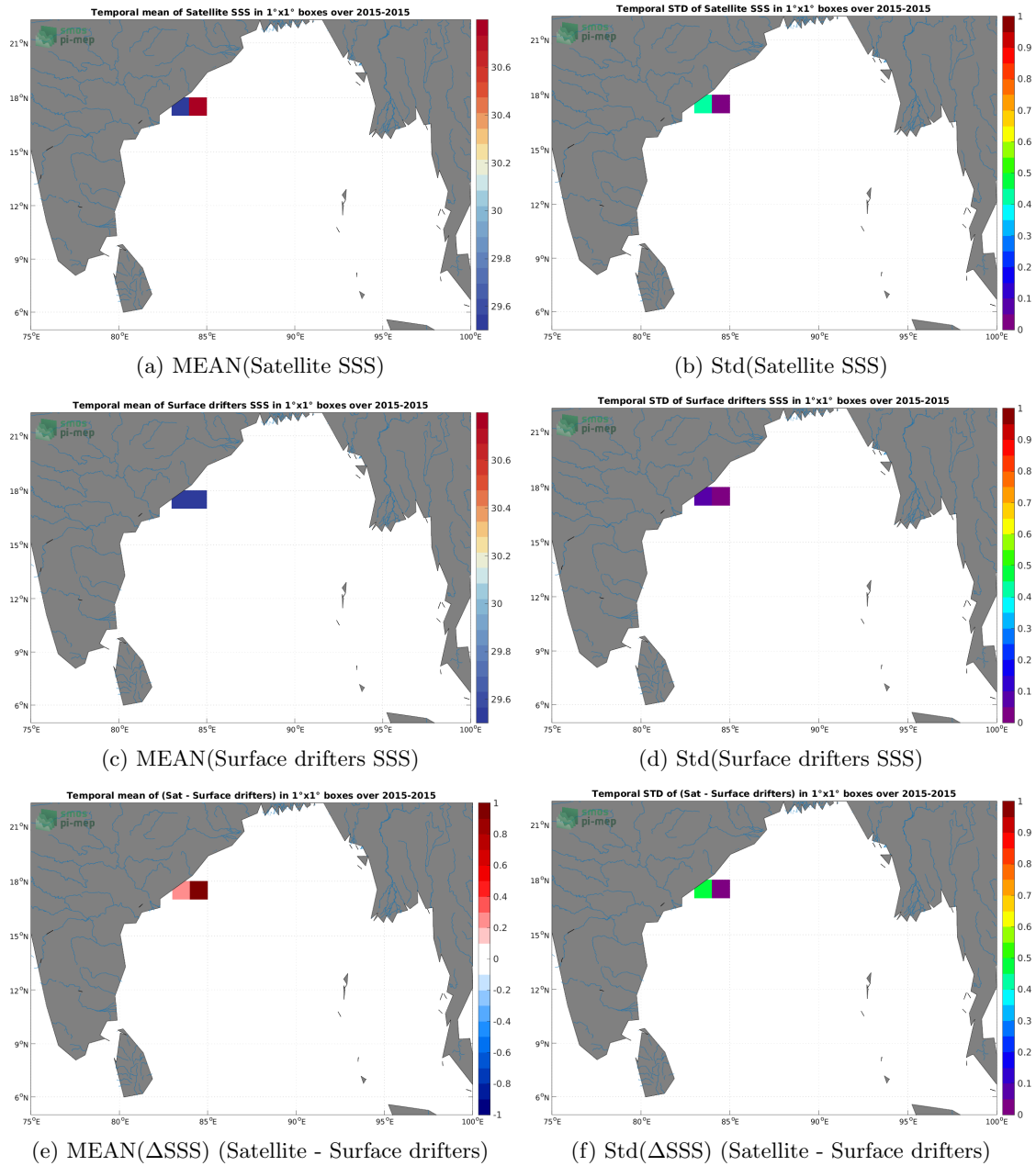
Figure 5: Temporal mean (left) and Std (right) of SSS from SMAP SSS L2 v5 - 40 km (RSS) (top), Surface drifters (middle), and of \Delta SSS (Satellite - Surface drifters). Only match-up pairs are used to generate these maps.
