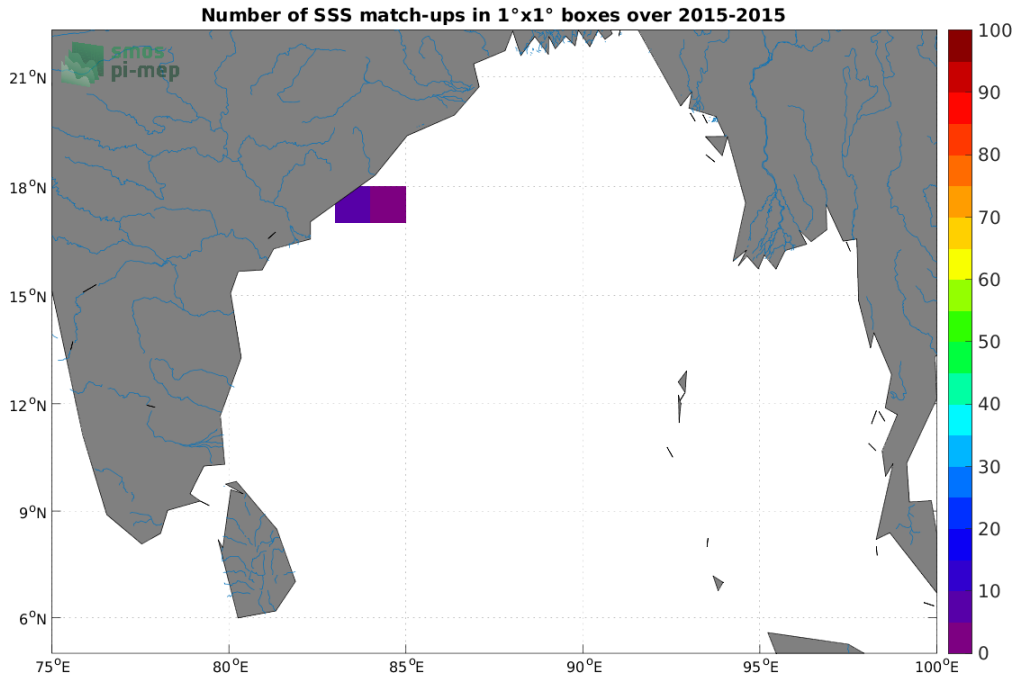
Figure 3: Number of SSS match-ups between Surface drifters SSS and the SMAP SSS L2 v5 - 40 km (RSS) SSS product for the Ganga and Brahmaputra river plumes Pi-MEP region over 1°×1° boxes and for the full satellite product period.
