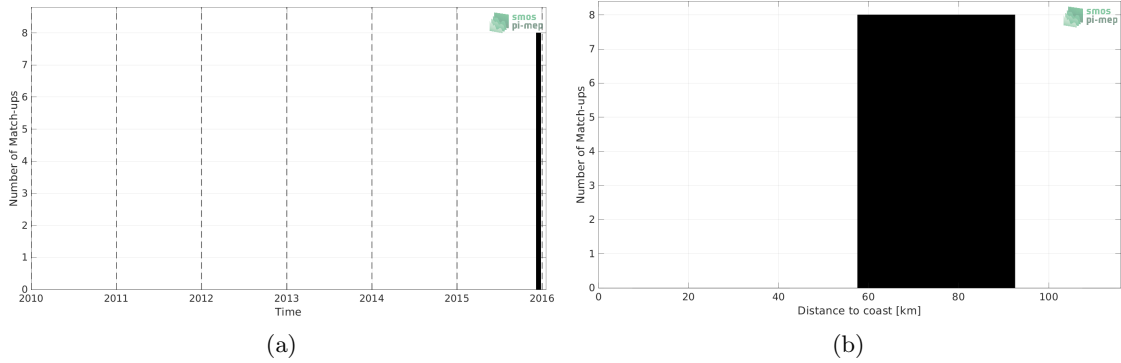
Figure 1: Number of match-ups between Surface drifters and SMAP SSS L2 v5 - 40 km (RSS) SSS as a function of time (a) and as function of the distance to coast (b) over the Ganga and Brahmaputra river plumes Pi-MEP region and for the full satellite product period.
