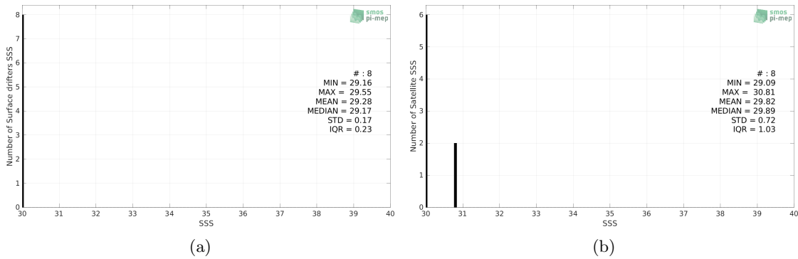
Figure 2: Histograms of SSS from Surface drifters (a) and SMAP SSS L2 v5 - 40 km (RSS) (b) considering all match-up pairs per bins of 0.1 over the Ganga and Brahmaputra river plumes Pi-MEP region and for the full satellite product period.
