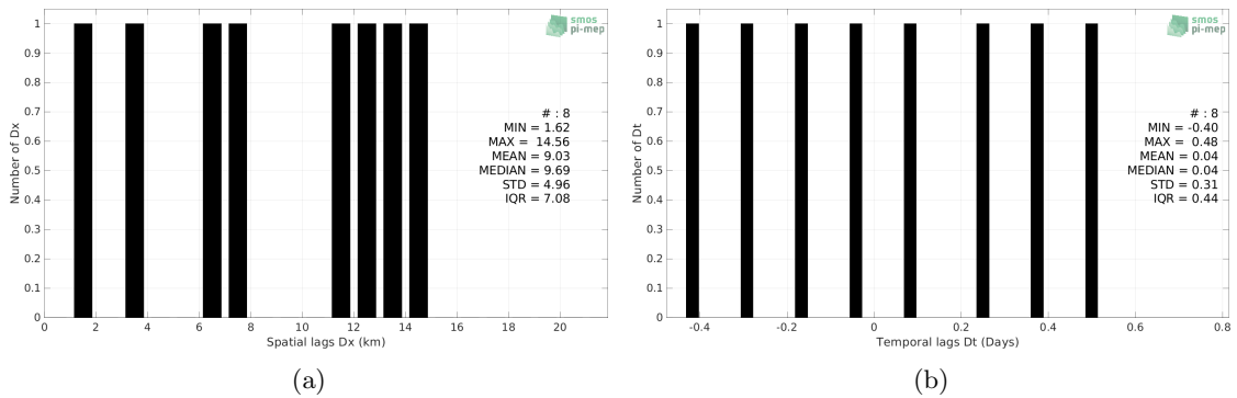
Figure 4: Histograms of the spatial (a) and temporal (b) lags between the location/time of the Surface drifters measurement and the date of the corresponding SMAP SSS L2 v5 - 40 km (RSS) SSS pixel.
