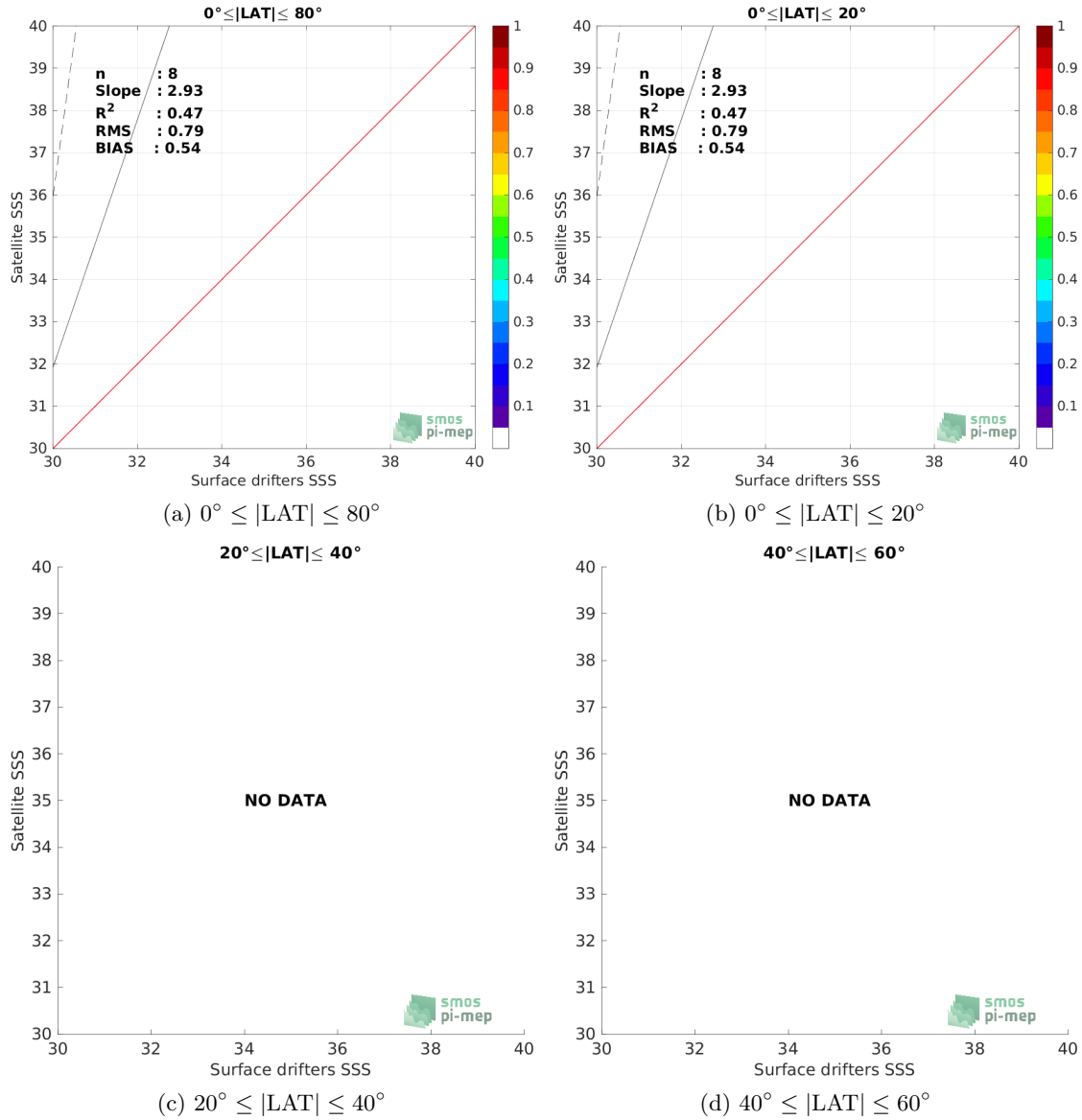
Figure 8: Contour maps of the concentration of SMAP SSS L2 v5 - 40 km (RSS) SSS (y-axis) versus Surface drifters SSS (x-axis) at match-up pairs for different latitude bands. For each plot, the red line shows x=y . The black thin and dashed lines indicate a linear fit through the data cloud and the \pm 95\% confidence levels, respectively. The number match-up pairs n , the slope and R^2 coefficient of the linear fit, the root mean square (RMS) and the mean bias between satellite and in situ data are indicated for each latitude band in each plots.
