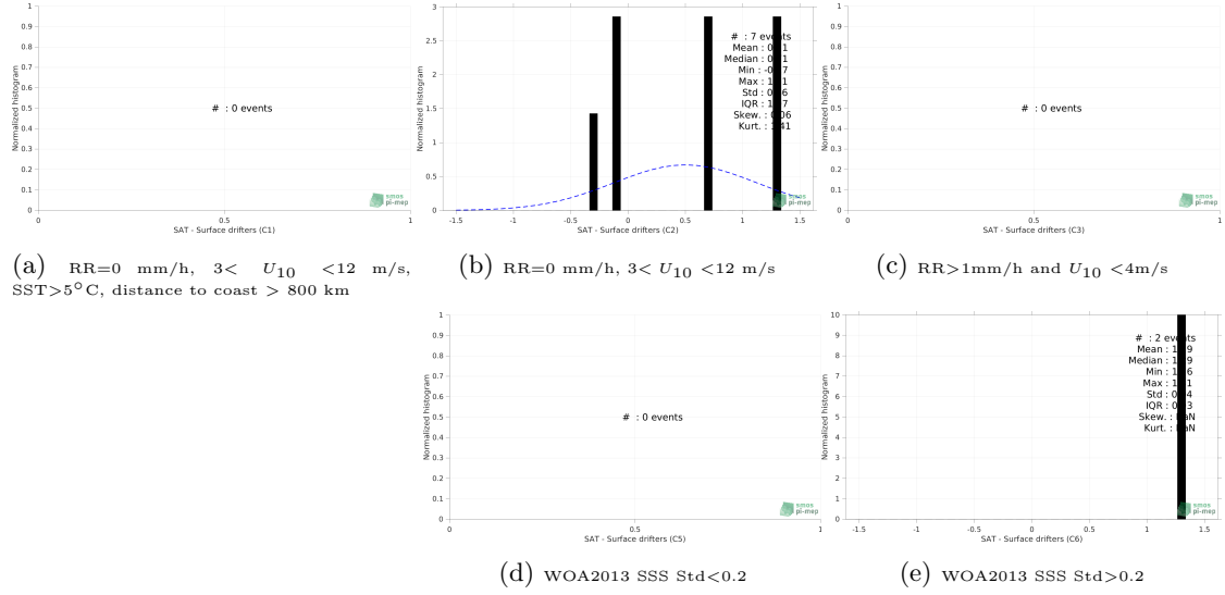
Figure 12: Normalized histogram of \Delta SSS (SMAP SSS L2 v5 - 40 km (RSS) - Surface drifters) for 5 different subdatasets corresponding to: RR=0 mm/h, 3 < U_{10} < 12 m/s, SST>5°C, distance to coast > 800 km (a), RR=0 mm/h, 3 < U_{10} < 12 m/s (b), RR>1mm/h and U_{10} < 4 m/s (c), WOA2013 SSS Std<0.2 (d), WOA2013 SSS Std>0.2 (e).
