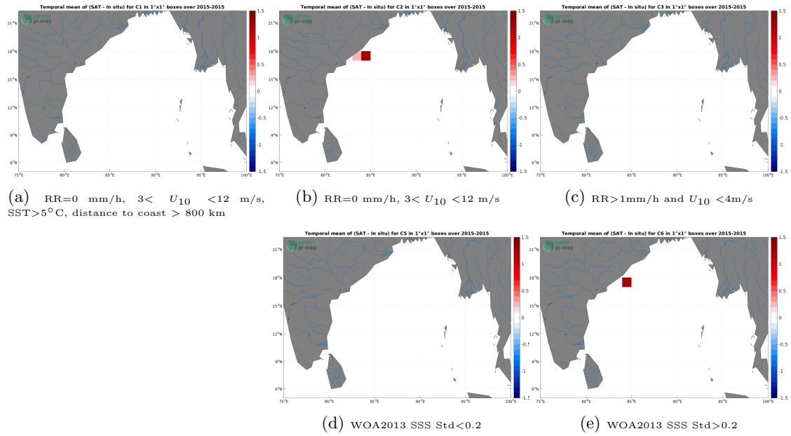
Figure 11: Temporal mean gridded over spatial boxes of size 1^\circ \times 1^\circ of \Delta SSS (SMAP SSS L2 v5 - 40 km (RSS) - Surface drifters) for 5 different subdatasets corresponding to:RR=0 mm/h, 3 < U_{10} < 12 m/s, SST >5^\circ C, distance to coast > 800 km (a), RR=0 mm/h, 3 < U_{10} < 12 m/s (b), RR >1 mm/h and U_{10} < 4 m/s (c), WOA2013 SSS Std <0.2 (d), WOA2013 SSS Std >0.2 (e).
