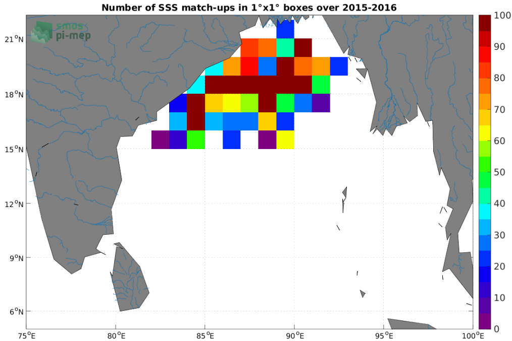
Figure 3: Number of SSS match-ups between Surface drifters SSS and the SMAP SSS L2 v5 - 40 km (RSS) SSS product for the Ganga and Brahmaputra river plumes Pi-MEP region over 1°x1° boxes and for the full satellite product period.
