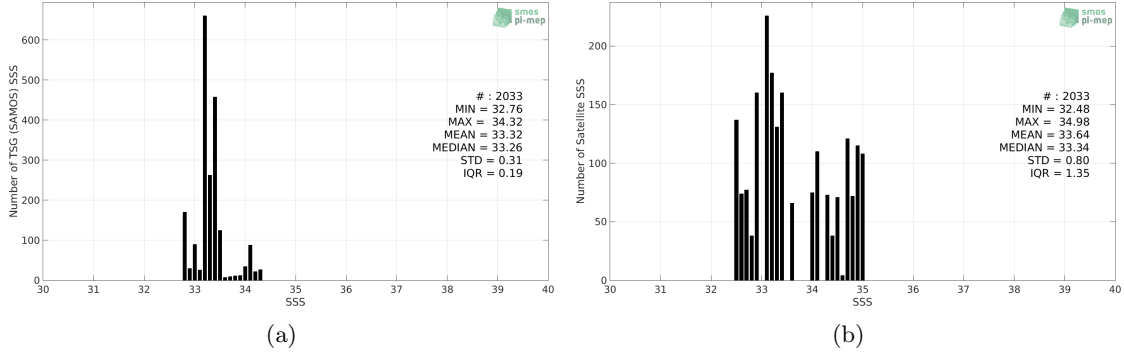
Figure 2: Histograms of SSS from TSG (SAMOS) (a) and SMAP SSS L2 v4 (RSS) (b) considering all match-up pairs per bins of 0.1 over the Ganga and Brahmaputra river plumes Pi-MEP region and for the full satellite product period.
