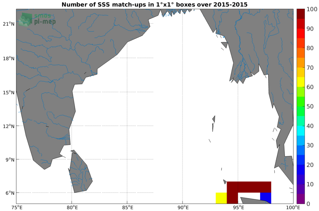
Figure 4: Number of SSS match-ups between TSG (SAMOS) SSS and the SMAP SSS L2 v4 (RSS) SSS product for the Ganga and Brahmaputra river plumes Pi-MEP region over 1^\circ \times 1^\circ boxes and for the full satellite product period.
