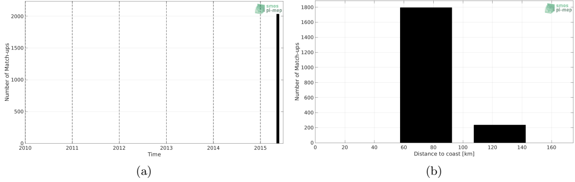
Figure 1: Number of match-ups between TSG (SAMOS) and SMAP SSS L2 v4 (RSS) SSS as a function of time (a) and as function of the distance to coast (b) over the Ganga and Brahmaputra river plumes Pi-MEP region and for the full satellite product period.
