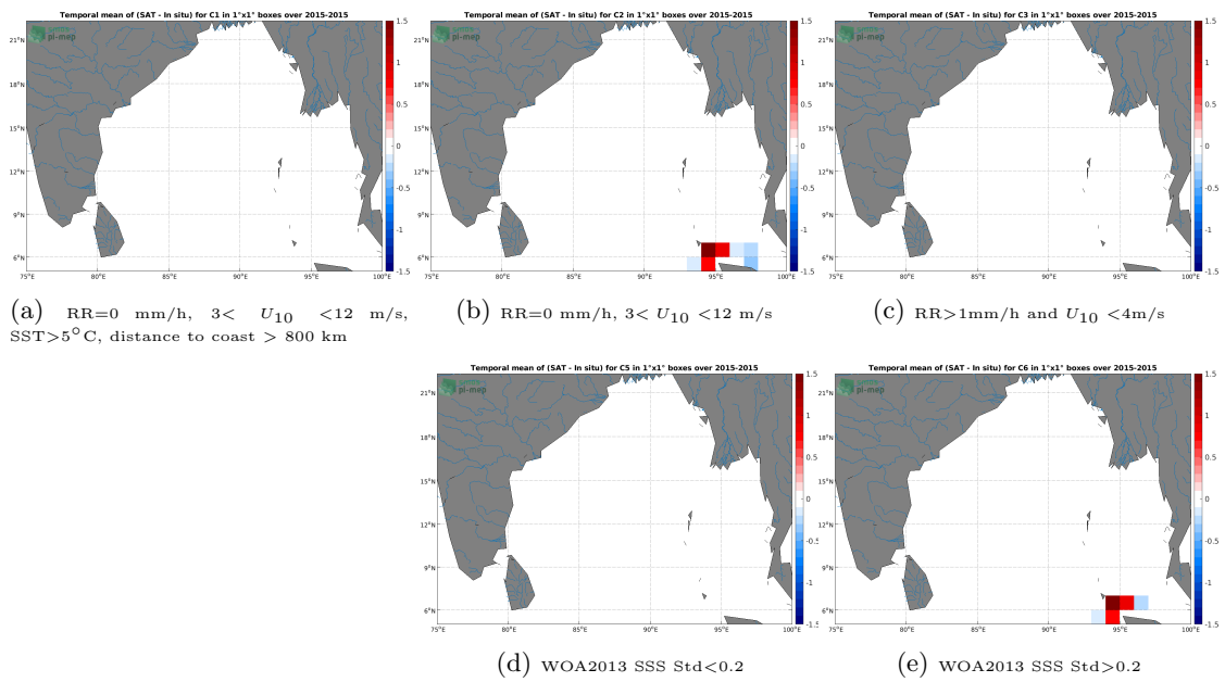
Figure 12: Temporal mean gridded over spatial boxes of size 1°x1° of \Delta SSS (SMAP SSS L2 v4 (RSS) - TSG (SAMOS)) for 5 different subdatasets corresponding to:RR=0 mm/h, 3 < U_{10} < 12 m/s, SST>5°C, distance to coast > 800 km (a), RR=0 mm/h, 3 < U_{10} < 12 m/s (b), RR>1mm/h and U_{10} < 4 m/s (c), WOA2013 SSS Std<0.2 (d), WOA2013 SSS Std>0.2 (e).
