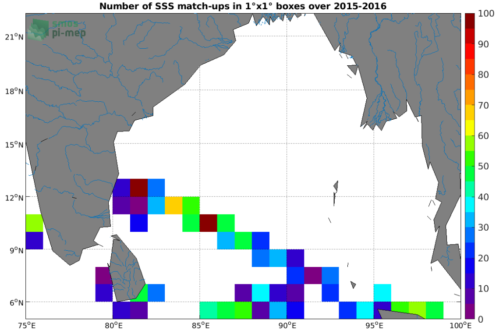
Figure 4: Number of SSS match-ups between TSG (LEGOS-DM) SSS and the SMAP SSS L2 v4 (RSS) SSS product for the Ganga and Brahmaputra river plumes Pi-MEP region over 1^\circ \times 1^\circ boxes and for the full satellite product period.
