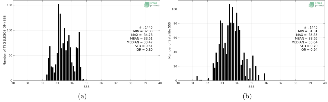
Figure 2: Histograms of SSS from TSG (LEGOS-DM) (a) and SMAP SSS L2 v4 (RSS) (b) considering all match-up pairs per bins of 0.1 over the Ganga and Brahmaputra river plumes Pi-MEP region and for the full satellite product period.
