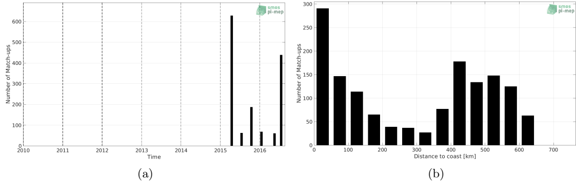
Figure 1: Number of match-ups between TSG (LEGOS-DM) and SMAP SSS L2 v4 (RSS) SSS as a function of time (a) and as function of the distance to coast (b) over the Ganga and Brahmaputra river plumes Pi-MEP region and for the full satellite product period.
