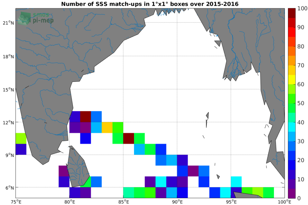
Figure 4: Number of SSS match-ups between TSG (LEGOS-DM) SSS and the SMAP SSS L2 v4 (RSS) SSS product for the Ganga and Brahmaputra river plumes Pi-MEP region over 1°x1° boxes and for the full satellite product period.
