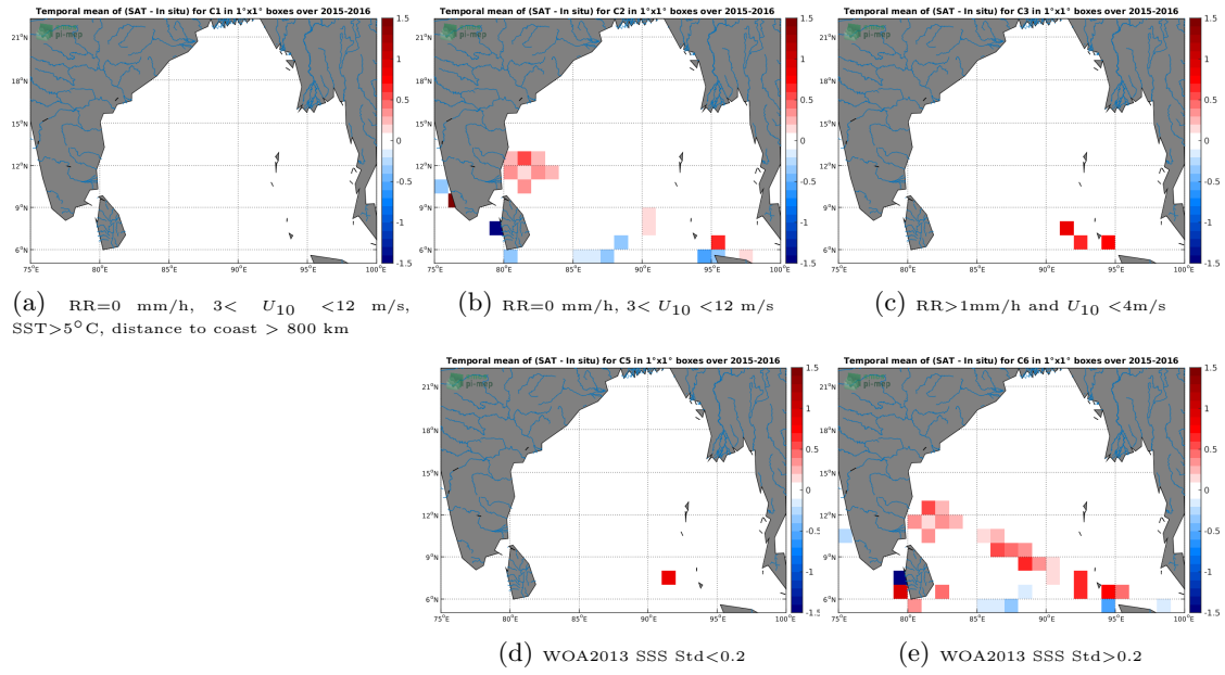
Figure 12: Temporal mean gridded over spatial boxes of size 1^\circ \times 1^\circ of \Delta SSS (SMAP-L2-RSS-V4 - TSG-LEGOS-DM) for 5 different subdatasets corresponding to: RR=0 mm/h, 3 < U_{10} < 12 m/s, SST > 5^\circ C , distance to coast > 800 km (a), RR=0 mm/h, 3 < U_{10} < 12 m/s (b), RR > 1 mm/h and U_{10} < 4 m/s (c), WOA2013 SSS Std < 0.2 (d), WOA2013 SSS Std > 0.2 (e).
