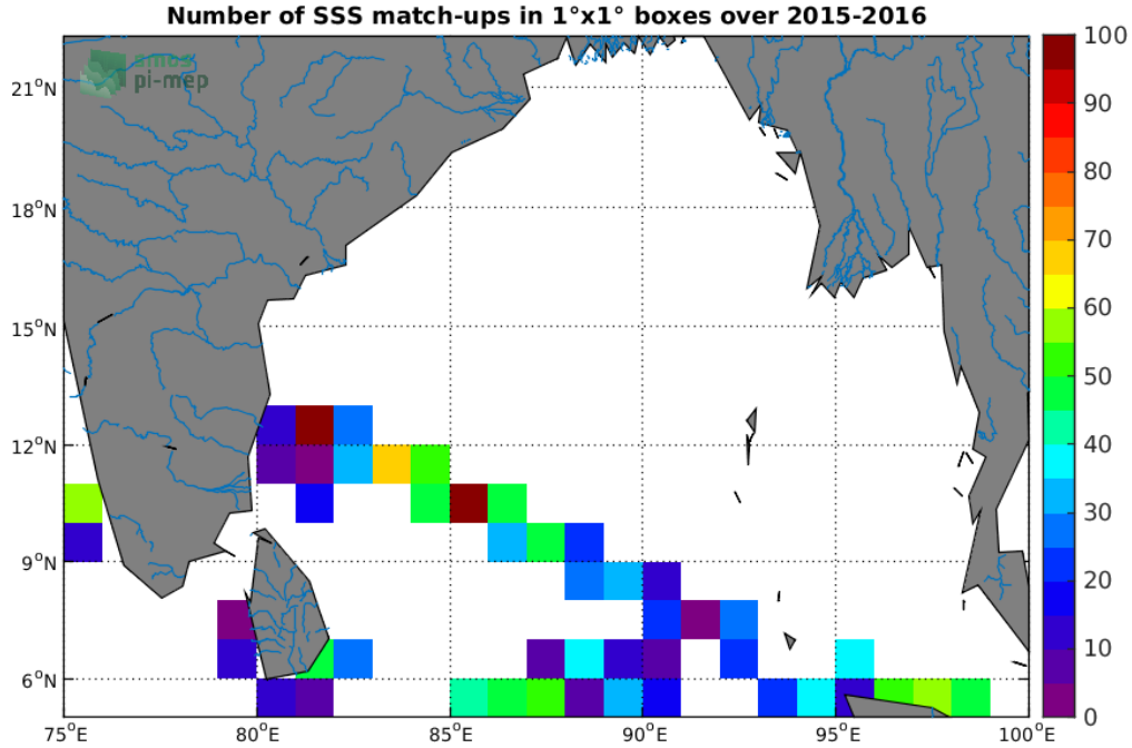
Figure 4: Number of SSS match-ups between TSG-LEGOS-DM SSS and the SMAP-L2-RSS-V4 SSS product for the Ganga and Brahmaputra river plumes Pi-MEP region over 1^\circ \times 1^\circ boxes and for the full satellite product period.
