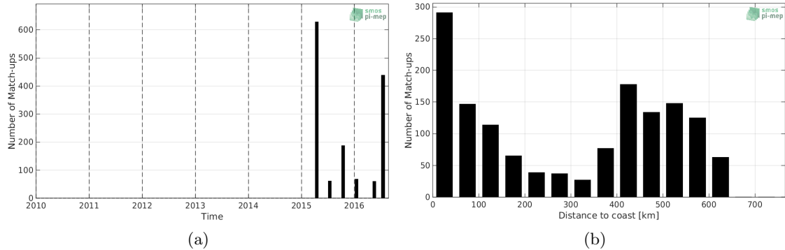
Figure 1: Number of match-ups between TSG-LEGOS-DM and SMAP-L2-RSS-V4 SSS as a function of time (a) and as function of the distance to coast (b) over the Ganga and Brahmaputra river plumes Pi-MEP region and for the full satellite product period.
