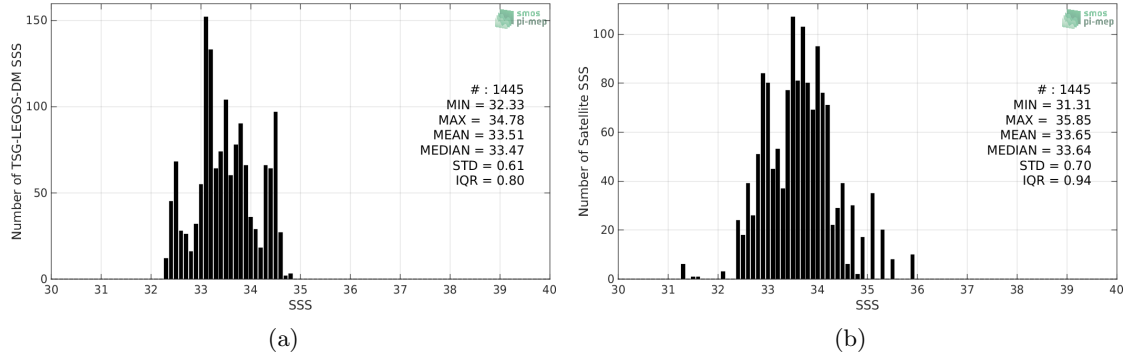
Figure 2: Histograms of SSS from TSG-LEGOS-DM (a) and SMAP-L2-RSS-V4 (b) considering all match-up pairs per bins of 0.1 over the Ganga and Brahmaputra river plumes Pi-MEP region and for the full satellite product period.
