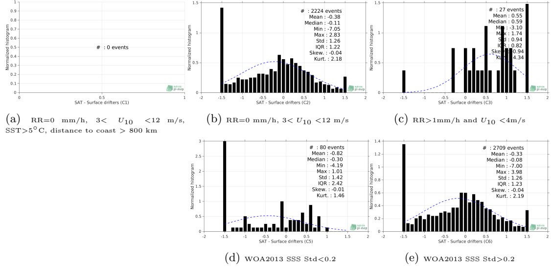
Figure 12: Normalized histogram of \Delta SSS (SMAP-L2-RSS-V4 - Surface drifters) for 5 different subdatasets corresponding to: RR=0 mm/h, 3 < U_{10} < 12 m/s, SST>5°C, distance to coast > 800 km (a), RR=0 mm/h, 3 < U_{10} < 12 m/s (b), RR>1mm/h and U_{10} < 4 m/s (c), WOA2013 SSS Std<0.2 (d), WOA2013 SSS Std>0.2 (e).
