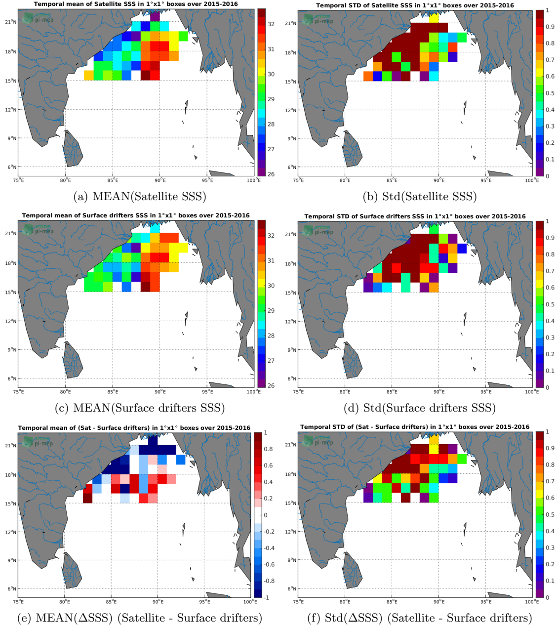
Figure 5: Temporal mean (left) and Std (right) of SSS from SMAP-L2-RSS-V4 (top), Surface drifters (middle), and of \Delta SSS (Satellite - Surface drifters). Only match-up pairs are used to generate these maps.
