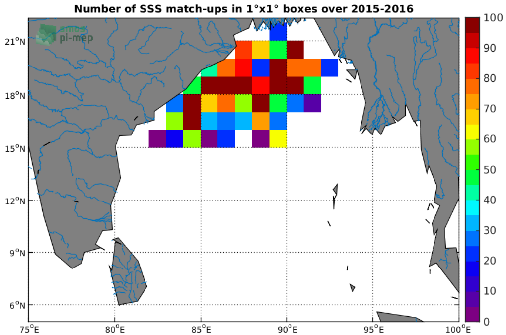
Figure 3: Number of SSS match-ups between Surface drifters SSS and the SMAP-L2-RSS-V4 SSS product for the Ganga and Brahmaputra river plumes Pi-MEP region over 1^\circ \times 1^\circ boxes and for the full satellite product period.
