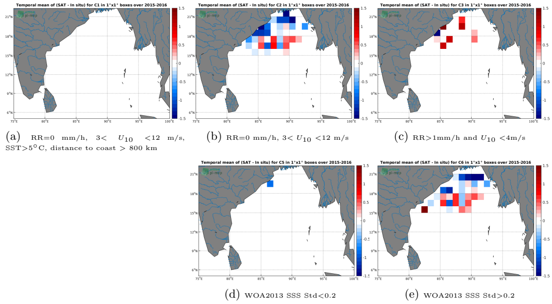
Figure 11: Temporal mean gridded over spatial boxes of size 1^\circ \times 1^\circ of \Delta SSS (SMAP-L2-RSS-V4 - Surface drifters) for 5 different subdatasets corresponding to: RR=0 mm/h, 3 < U_{10} < 12 m/s, SST > 5^\circ C , distance to coast > 800 km (a), RR=0 mm/h, 3 < U_{10} < 12 m/s (b), RR > 1 mm/h and U_{10} < 4 m/s (c), WOA2013 SSS Std < 0.2 (d), WOA2013 SSS Std > 0.2 (e).
