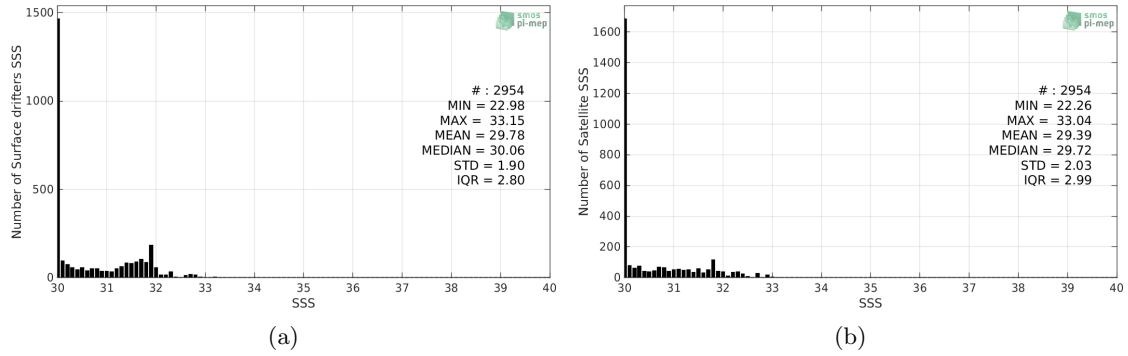
Figure 2: Histograms of SSS from Surface drifters (a) and SMAP-L2-RSS-V4 (b) considering all match-up pairs per bins of 0.1 over the Ganga and Brahmaputra river plumes Pi-MEP region and for the full satellite product period.
