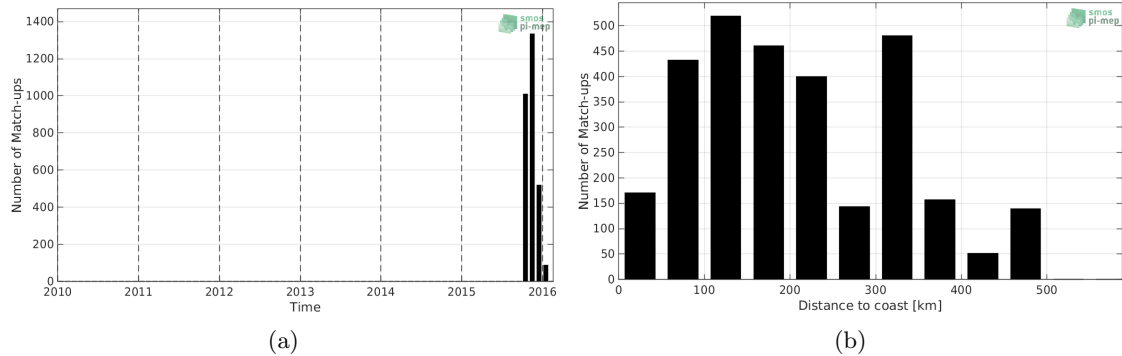
Figure 1: Number of match-ups between Surface drifters and SMAP-L2-RSS-V4 SSS as a function of time (a) and as function of the distance to coast (b) over the Ganga and Brahmaputra river plumes Pi-MEP region and for the full satellite product period.
