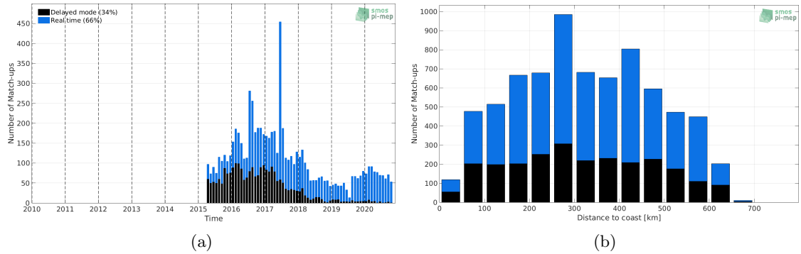
Figure 1: Number of match-ups between Argo and SMAP SSS L2 v4 (RSS) SSS as a function of time (a) and as function of the distance to coast (b) over the Ganga and Brahmaputra river plumes Pi-MEP region and for the full satellite product period.
