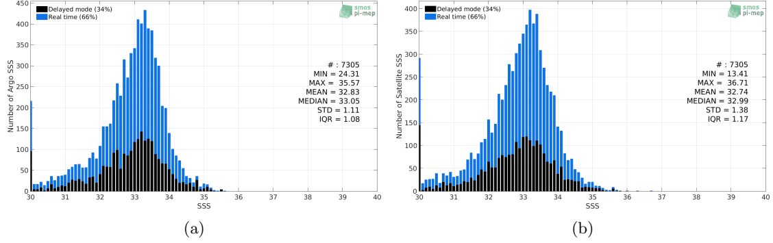
Figure 2: Histograms of SSS from Argo (a) and SMAP SSS L2 v4 (RSS) (b) considering all match-up pairs per bins of 0.1 over the Ganga and Brahmaputra river plumes Pi-MEP region and for the full satellite product period.
