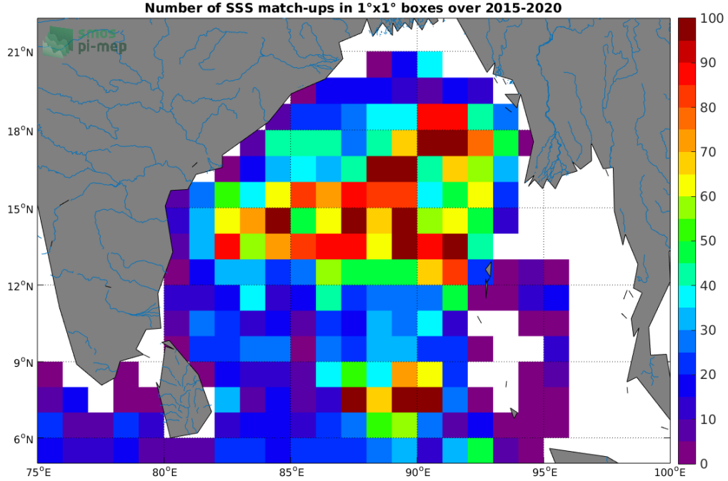
Figure 4: Number of SSS match-ups between Argo SSS and the SMAP SSS L2 v4 (RSS) SSS product for the Ganga and Brahmaputra river plumes Pi-MEP region over 1^\circ \times 1^\circ boxes and for the full satellite product period.
