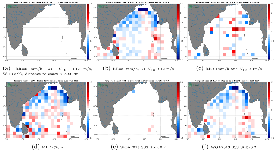
Figure 12: Temporal mean gridded over spatial boxes of size 1^\circ \times 1^\circ of \Delta SSS (SMAP SSS L2 v4 (RSS) - Argo) for 6 different subdatasets corresponding to:RR=0 mm/h, 3 < U_{10} < 12 m/s, SST >5^\circ\text{C} , distance to coast > 800 km (a), RR=0 mm/h, 3 < U_{10} < 12 m/s (b), RR >1 mm/h and U_{10} < 4 m/s (c),MLD <20 m (d),WOA2013 SSS Std <0.2 (e),WOA2013 SSS Std >0.2 (f).
