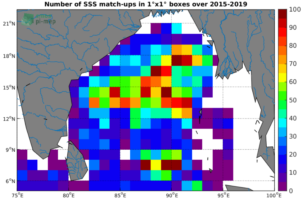
Figure 4: Number of SSS match-ups between Argo SSS and the SMAP-L2-RSS-V4 SSS product for the Ganga and Brahmaputra river plumes Pi-MEP region over 1^\circ \times 1^\circ boxes and for the full satellite product period.
