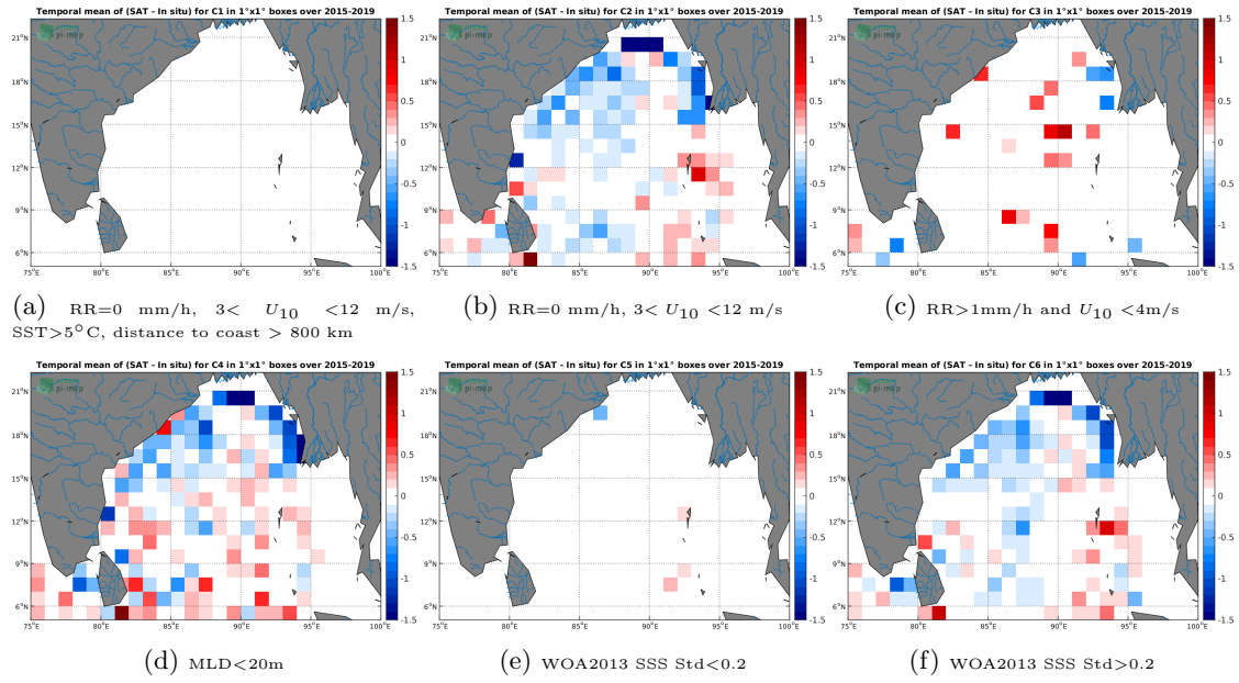
Figure 12: Temporal mean gridded over spatial boxes of size 1^\circ \times 1^\circ of \Delta SSS (SMAP-L2-RSS-V4 - Argo) for 6 different subdatasets corresponding to: RR=0 mm/h, 3 < U_{10} < 12 m/s, SST > 5^\circ C , distance to coast > 800 km (a), RR=0 mm/h, 3 < U_{10} < 12 m/s (b), RR > 1 mm/h and U_{10} < 4 m/s (c), MLD < 20 m (d), WOA2013 SSS Std < 0.2 (e), WOA2013 SSS Std > 0.2 (f).
