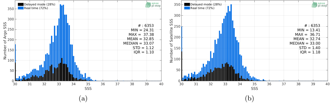
Figure 2: Histograms of SSS from Argo (a) and SMAP-L2-RSS-V4 (b) considering all match-up pairs per bins of 0.1 over the Ganga and Brahmaputra river plumes Pi-MEP region and for the full satellite product period.
