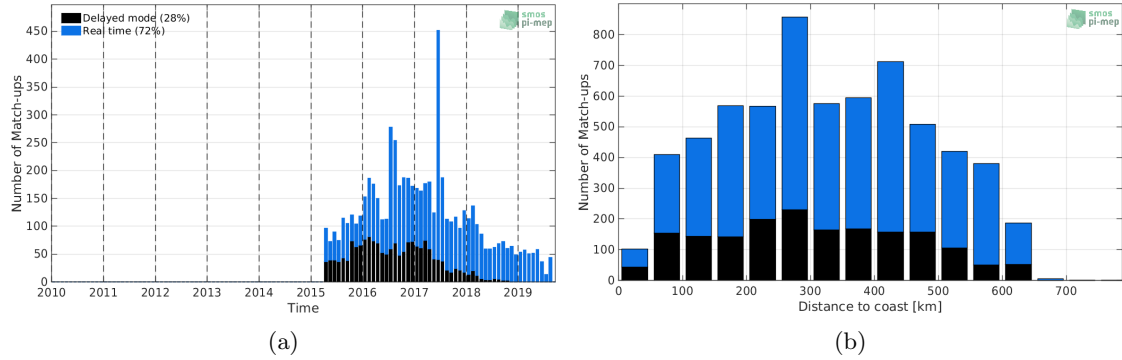
Figure 1: Number of match-ups between Argo and SMAP-L2-RSS-V4 SSS as a function of time (a) and as function of the distance to coast (b) over the Ganga and Brahmaputra river plumes Pi-MEP region and for the full satellite product period.
