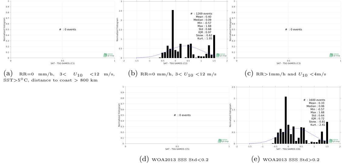
Figure 13: Normalized histogram of \Delta\text{SSS} (SMAP-L2-RSS-V3-70KM - TSG-SAMOS) for 5 different subdatasets corresponding to: RR=0 mm/h, 3 < U_{10} < 12 m/s, SST > 5^\circ\text{C} , distance to coast > 800 km (a), RR=0 mm/h, 3 < U_{10} < 12 m/s (b), RR > 1 mm/h and U_{10} < 4 m/s (c), WOA2013 SSS Std < 0.2 (d), WOA2013 SSS Std > 0.2 (e).
