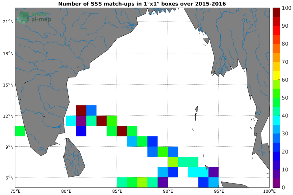
Figure 4: Number of SSS match-ups between TSG-LEGOS-DM SSS and the SMAP-L2-RSS-V3-70KM SSS product for the Ganga and Brahmaputra river plumes Pi-MEP region over 1^\circ \times 1^\circ boxes and for the full satellite product period.
