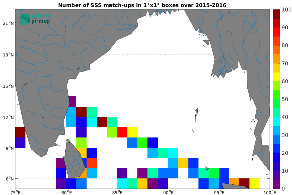
Figure 4: Number of SSS match-ups between TSG (LEGOS-DM) SSS and the SMAP SSS L2 v5.0 (JPL) SSS product for the Ganga and Brahmaputra river plumes Pi-MEP region over 1^{\circ} \times 1^{\circ} boxes and for the full satellite product period.
