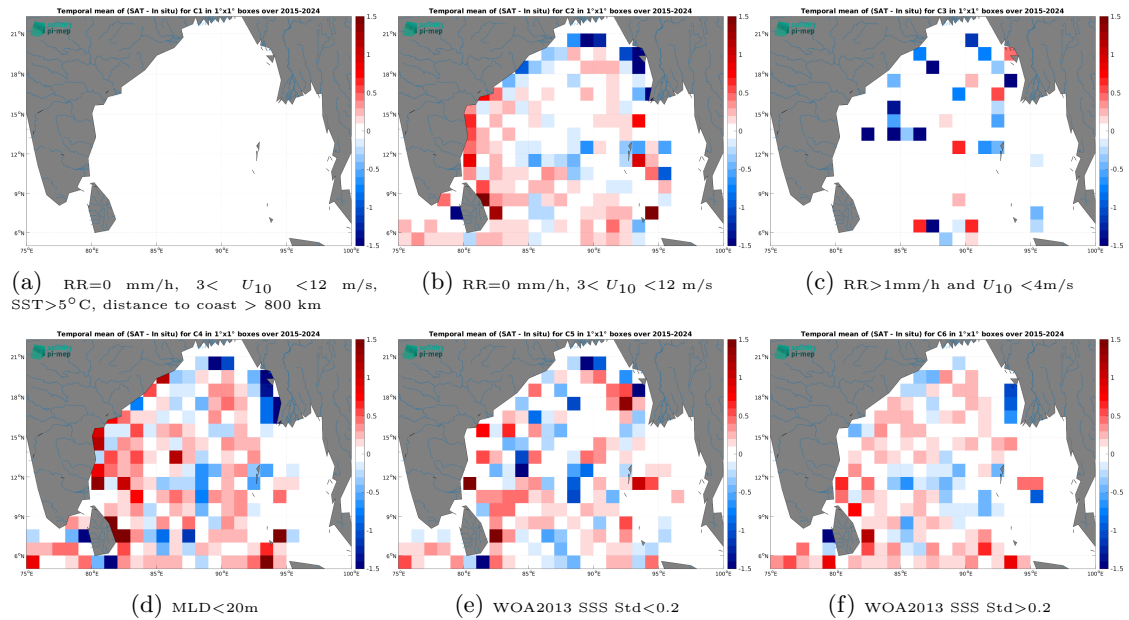
Figure 14: Temporal mean gridded over spatial boxes of size 1^\circ \times 1^\circ of \Delta SSS (SMAP SSS L2 v5.0 (JPL) - Argo) for 6 different subdatasets corresponding to:RR=0 mm/h, 3 < U_{10} < 12 m/s, SST>5°C, distance to coast > 800 km (a), RR=0 mm/h, 3 < U_{10} < 12 m/s (b), RR>1mm/h and U_{10} < 4 m/s (c),MLD<20m (d),WOA2013 SSS Std<0.2 (e),WOA2013 SSS Std>0.2 (f).
