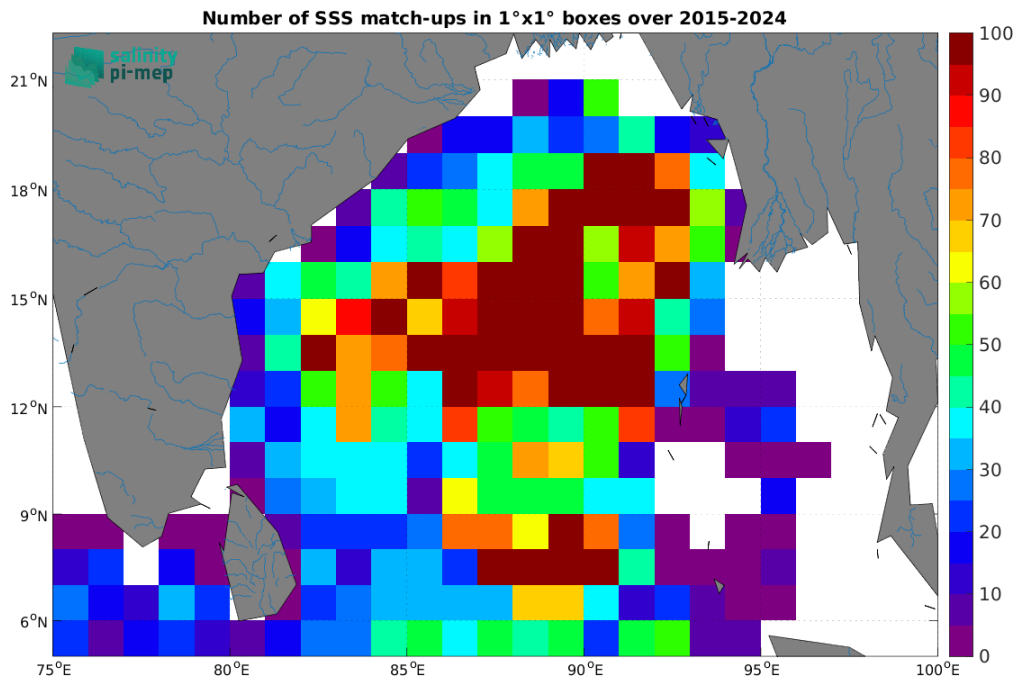
Figure 5: Number of SSS match-ups between Argo SSS and the SMAP SSS L2 v5.0 (JPL) SSS product for the Ganga and Brahmaputra river plumes Pi-MEP region over 1^\circ \times 1^\circ boxes and for the full satellite product period.
