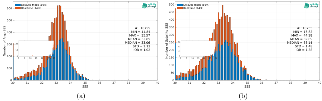
Figure 3: Histograms of SSS from Argo (a) and SMAP SSS L2 v5.0 (JPL) (b) considering all match-up pairs per bins of 0.1 over the Ganga and Brahmaputra river plumes Pi-MEP region and for the full satellite product period.
