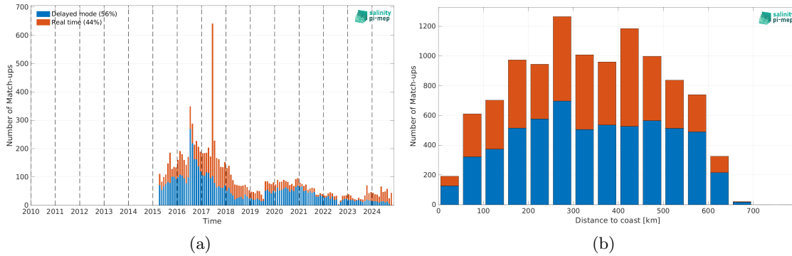
Figure 2: Number of match-ups between Argo and SMAP SSS L2 v5.0 (JPL) SSS as a function of time (a) and as function of the distance to coast (b) over the Ganga and Brahmaputra river plumes Pi-MEP region and for the full satellite product period.
