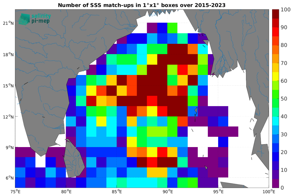
Figure 4: Number of SSS match-ups between Argo SSS and the SMAP SSS L2 v5.0 (JPL) SSS product for the Ganga and Brahmaputra river plumes Pi-MEP region over 1^\circ \times 1^\circ boxes and for the full satellite product period.
