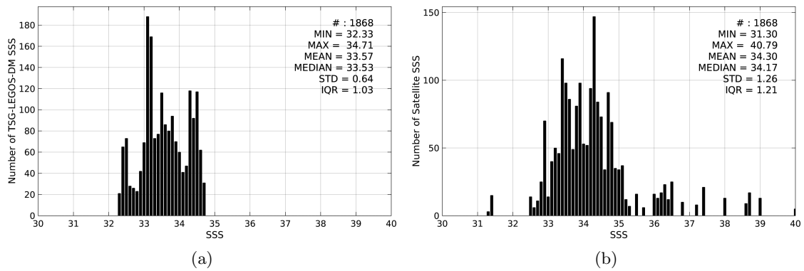
Figure 2: Histograms of SSS from TSG-LEGOS-DM (a) and SMAP-L2-JPL-V4 (b) considering all match-up pairs per bins of 0.1 over the Ganga and Brahmaputra river plumes Pi-MEP region and for the full satellite product period.
