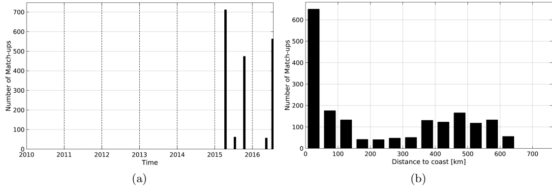
Figure 1: Number of match-ups between TSG-LEGOS-DM and SMAP-L2-JPL-V4 SSS as a function of time (a) and as function of the distance to coast (b) over the Ganga and Brahmaputra river plumes Pi-MEP region and for the full satellite product period.
