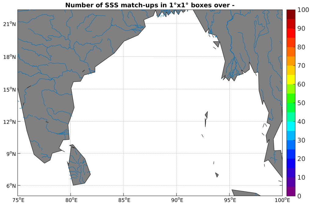
Figure 3: Number of SSS match-ups between Surface drifters SSS and the SMAP-L2-JPL-V4 SSS product for the Ganga and Brahmaputra river plumes Pi-MEP region over 1^\circ \times 1^\circ boxes and for the full satellite product period.
