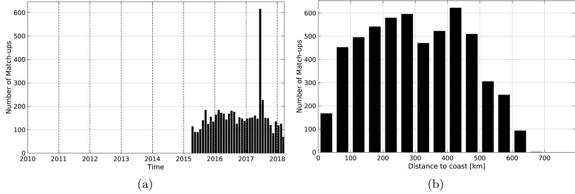
Figure 1: Number of match-ups between Argo and SMAP-L2-JPL-V4 SSS as a function of time (a) and as function of the distance to coast (b) over the Ganga and Brahmaputra river plumes Pi-MEP region and for the full satellite product period.
