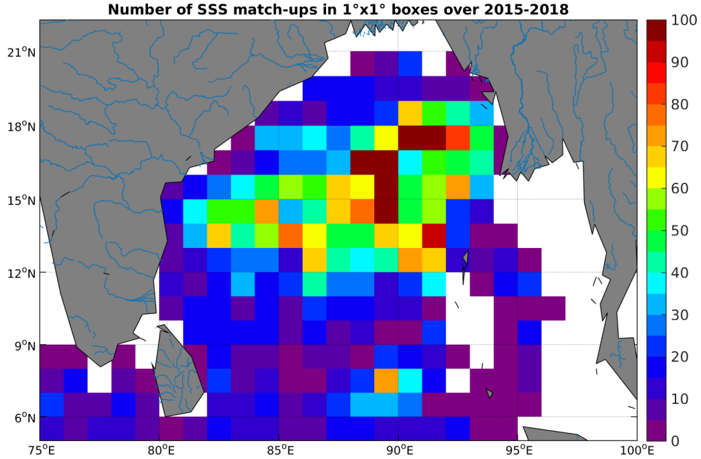
Figure 4: Number of SSS match-ups between Argo SSS and the SMAP-L2-JPL-V4 SSS product for the Ganga and Brahmaputra river plumes Pi-MEP region over 1^\circ \times 1^\circ boxes and for the full satellite product period.
