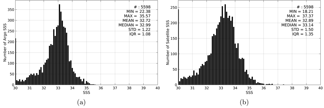
Figure 2: Histograms of SSS from Argo (a) and SMAP-L2-JPL-V4 (b) considering all match-up pairs per bins of 0.1 over the Ganga and Brahmaputra river plumes Pi-MEP region and for the full satellite product period.
