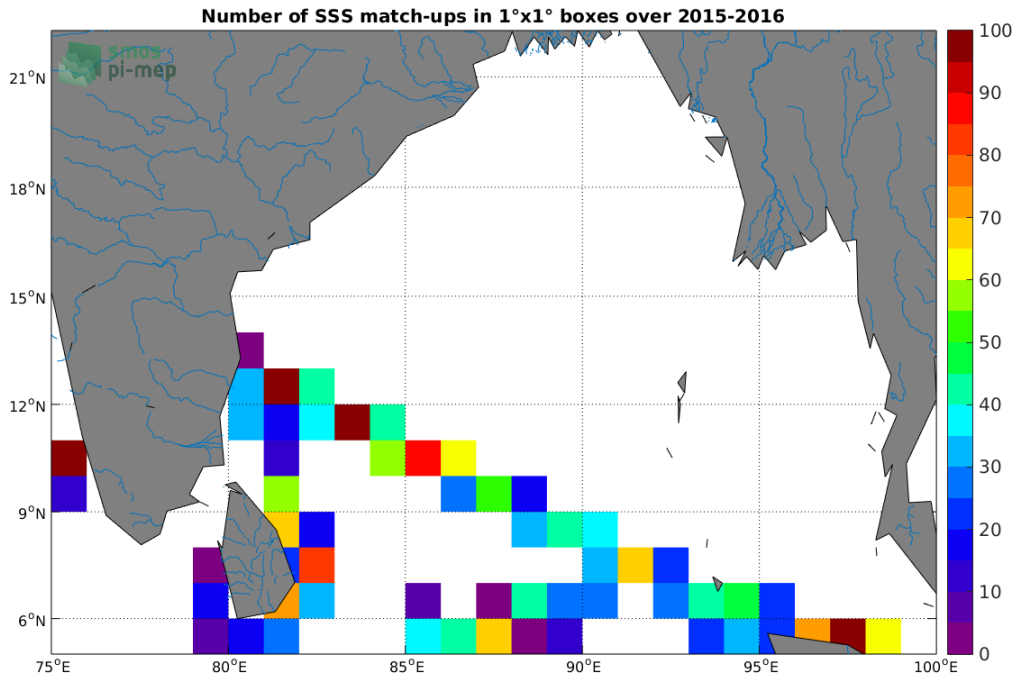
Figure 4: Number of SSS match-ups between TSG-LEGOS-DM SSS and the SMAP-L2-JPL-V4.3 SSS product for the Ganga and Brahmaputra river plumes Pi-MEP region over 1^\circ \times 1^\circ boxes and for the full satellite product period.
