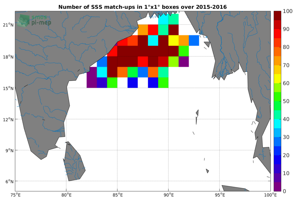
Figure 3: Number of SSS match-ups between Surface drifters SSS and the SMAP-L2-JPL-V4.3 SSS product for the Ganga and Brahmaputra river plumes Pi-MEP region over 1°x1° boxes and for the full satellite product period.
