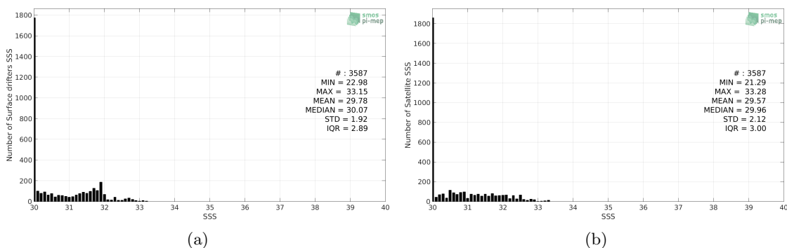
Figure 2: Histograms of SSS from Surface drifters (a) and SMAP-L2-JPL-V4.3 (b) considering all match-up pairs per bins of 0.1 over the Ganga and Brahmaputra river plumes Pi-MEP region and for the full satellite product period.
