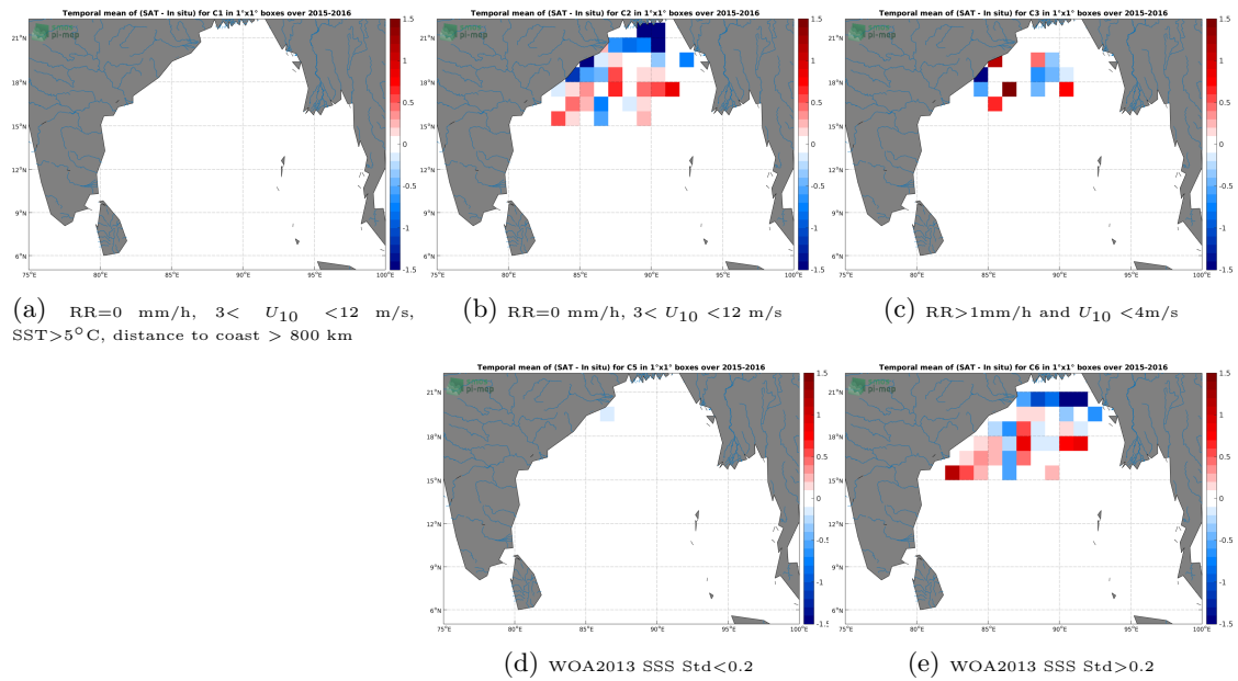
Figure 11: Temporal mean gridded over spatial boxes of size 1^\circ \times 1^\circ of \Delta SSS (SMAP-L2-JPL-V4.3 - Surface drifters) for 5 different subdatasets corresponding to:RR=0 mm/h, 3 < U_{10} < 12 m/s, SST >5^\circ C, distance to coast > 800 km (a), RR=0 mm/h, 3 < U_{10} < 12 m/s (b), RR >1 mm/h and U_{10} < 4 m/s (c), WOA2013 SSS Std <0.2 (d), WOA2013 SSS Std >0.2 (e).
