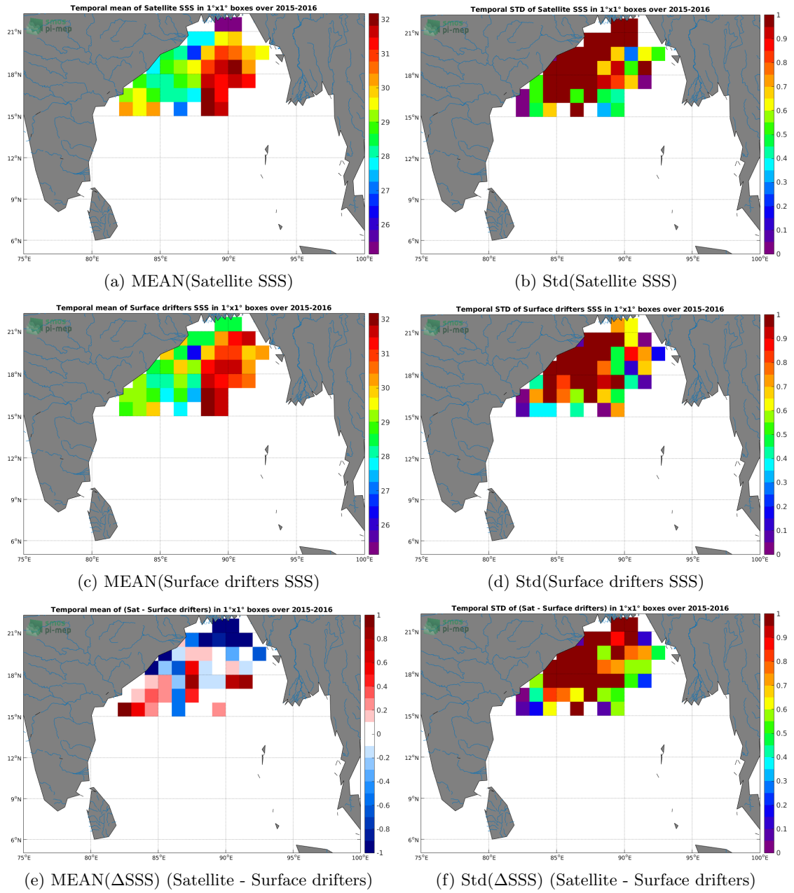
Figure 5: Temporal mean (left) and Std (right) of SSS from SMAP-L2-JPL-V4.3 (top), Surface drifters (middle), and of \Delta SSS (Satellite - Surface drifters). Only match-up pairs are used to generate these maps.
