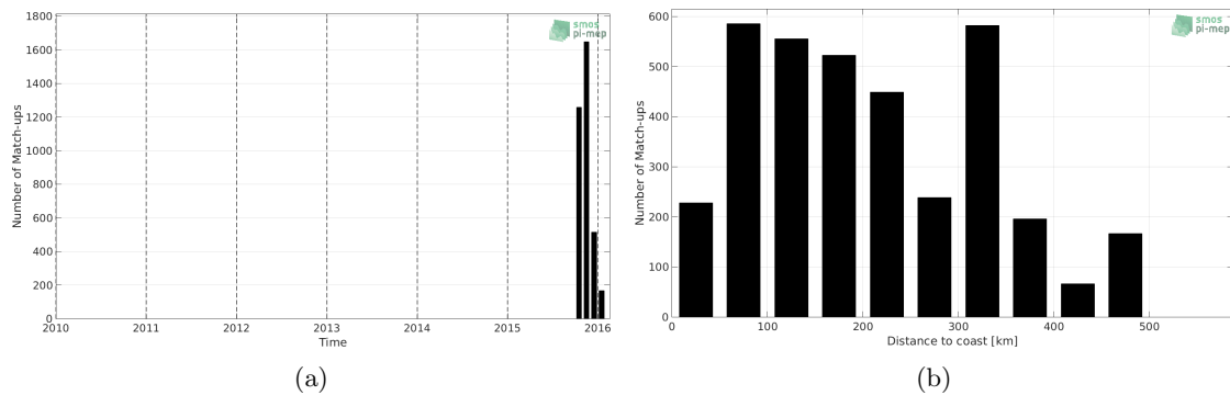
Figure 1: Number of match-ups between Surface drifters and SMAP-L2-JPL-V4.3 SSS as a function of time (a) and as function of the distance to coast (b) over the Ganga and Brahmaputra river plumes Pi-MEP region and for the full satellite product period.
