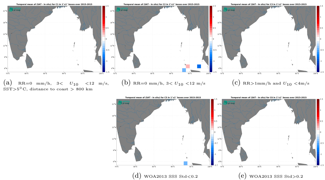
Figure 14: Temporal mean gridded over spatial boxes of size 1^\circ \times 1^\circ of \Delta SSS (ISAS v7 - Monthly (Ifremer-LOPS-CMEMS) - TSG (SAMOS)) for 5 different subdatasets corresponding to:RR=0 mm/h, 3 < U_{10} < 12 m/s, SST >5^\circ C, distance to coast > 800 km (a), RR=0 mm/h, 3 < U_{10} < 12 m/s (b), RR >1 mm/h and U_{10} < 4 m/s (c), WOA2013 SSS Std <0.2 (d), WOA2013 SSS Std >0.2 (e).
