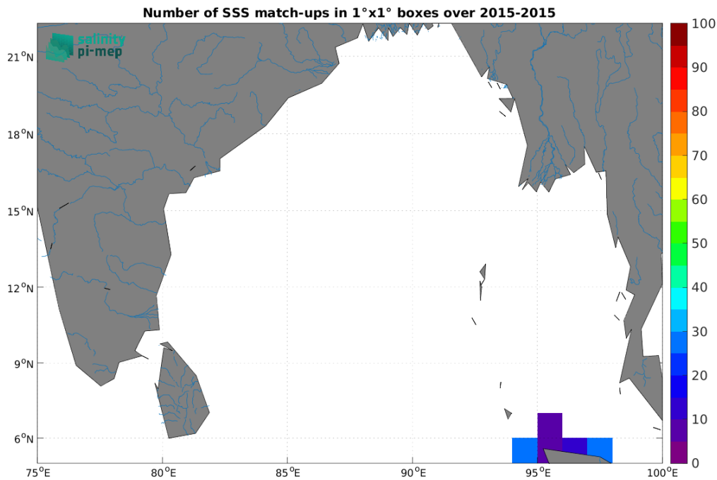
Figure 5: Number of SSS match-ups between TSG (SAMOS) SSS and the ISAS v7 - Monthly (Ifremer-LOPS-CMEMS) SSS product for the Ganga and Brahmaputra river plumes Pi-MEP region over 1^{\circ} \times 1^{\circ} boxes and for the full satellite product period.
