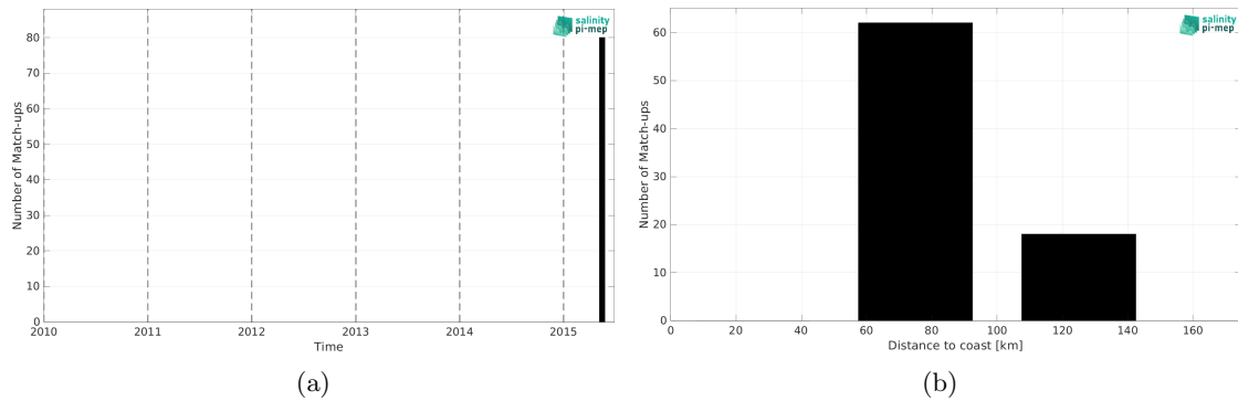
Figure 2: Number of match-ups between TSG (SAMOS) and ISAS v7 - Monthly (Ifremer-LOPS-CMEMS) SSS as a function of time (a) and as function of the distance to coast (b) over the Ganga and Brahmaputra river plumes Pi-MEP region and for the full satellite product period.
