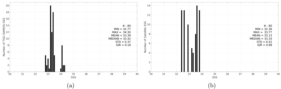
Figure 3: Histograms of SSS from TSG (SAMOS) (a) and ISAS v7 - Monthly (Ifremer-LOPS-CMEMS) (b) considering all match-up pairs per bins of 0.1 over the Ganga and Brahmaputra river plumes Pi-MEP region and for the full satellite product period.
