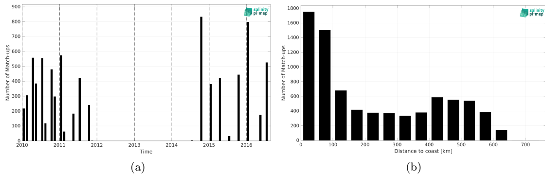
Figure 2: Number of match-ups between TSG (LEGOS-DM) and ISAS v7 - Monthly (Ifremer-LOPS-CMEMS) SSS as a function of time (a) and as function of the distance to coast (b) over the Ganga and Brahmaputra river plumes Pi-MEP region and for the full satellite product period.
