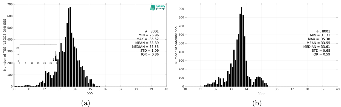
Figure 3: Histograms of SSS from TSG (LEGOS-DM) (a) and ISAS v7 - Monthly (Ifremer-LOPS-CMEMS) (b) considering all match-up pairs per bins of 0.1 over the Ganga and Brahmaputra river plumes Pi-MEP region and for the full satellite product period.
