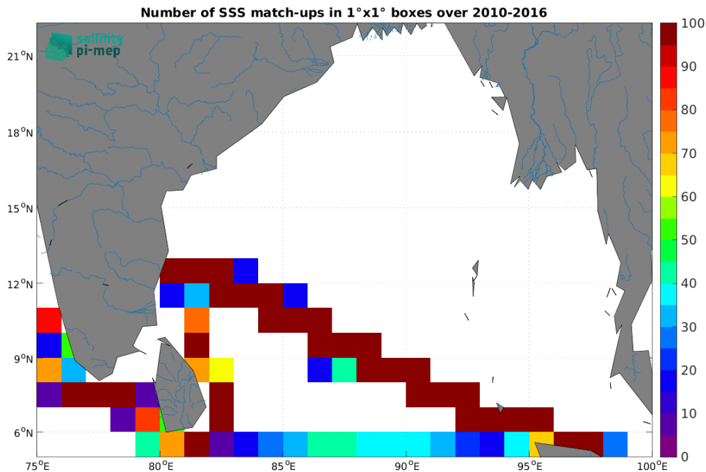
Figure 5: Number of SSS match-ups between TSG (LEGOS-DM) SSS and the ISAS v7 - Monthly (Ifremer-LOPS-CMEMS) SSS product for the Ganga and Brahmaputra river plumes Pi-MEP region over 1^\circ \times 1^\circ boxes and for the full satellite product period.
