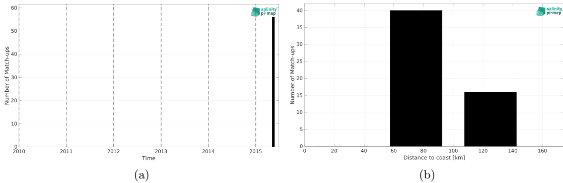
Figure 2: Number of match-ups between TSG (SAMOS) and CCI SSS L4 Merged-OI v4.41 - 7-day running (ESA) SSS as a function of time (a) and as function of the distance to coast (b) over the Ganga and Brahmaputra river plumes Pi-MEP region and for the full satellite product period.
