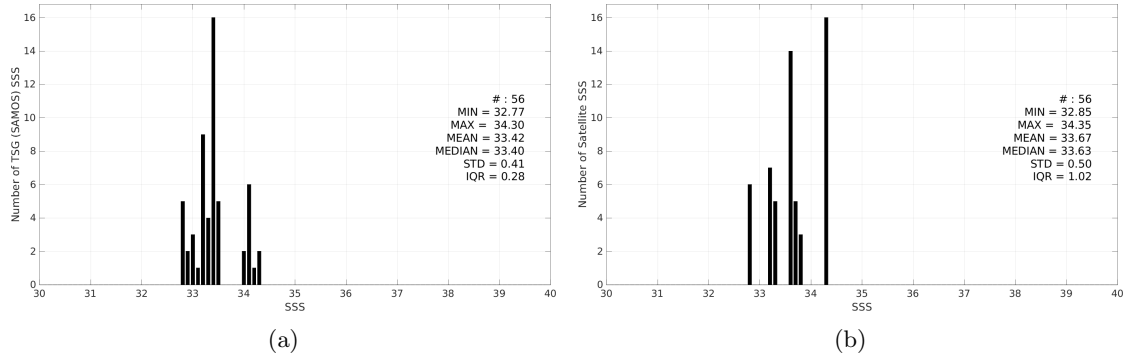
Figure 3: Histograms of SSS from TSG (SAMOS) (a) and CCI SSS L4 Merged-OI v4.41 - 7-day running (ESA) (b) considering all match-up pairs per bins of 0.1 over the Ganga and Brahmaputra river plumes Pi-MEP region and for the full satellite product period.
