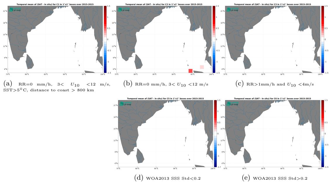
Figure 14: Temporal mean gridded over spatial boxes of size 1^\circ \times 1^\circ of \Delta SSS (CCI SSS L4 Merged-OI v4.41 - 7-day running (ESA) - TSG (SAMOS)) for 5 different subdatasets corresponding to:RR=0 mm/h, 3 < U_{10} < 12 m/s, SST>5°C, distance to coast > 800 km (a), RR=0 mm/h, 3 < U_{10} < 12 m/s (b), RR>1mm/h and U_{10} < 4 m/s (c), WOA2013 SSS Std<0.2 (d), WOA2013 SSS Std>0.2 (e).
