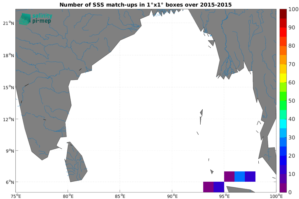
Figure 5: Number of SSS match-ups between TSG (SAMOS) SSS and the CCI SSS L4 Merged-OI v4.41 - 7-day running (ESA) SSS product for the Ganga and Brahmaputra river plumes Pi-MEP region over 1^{\circ} \times 1^{\circ} boxes and for the full satellite product period.
