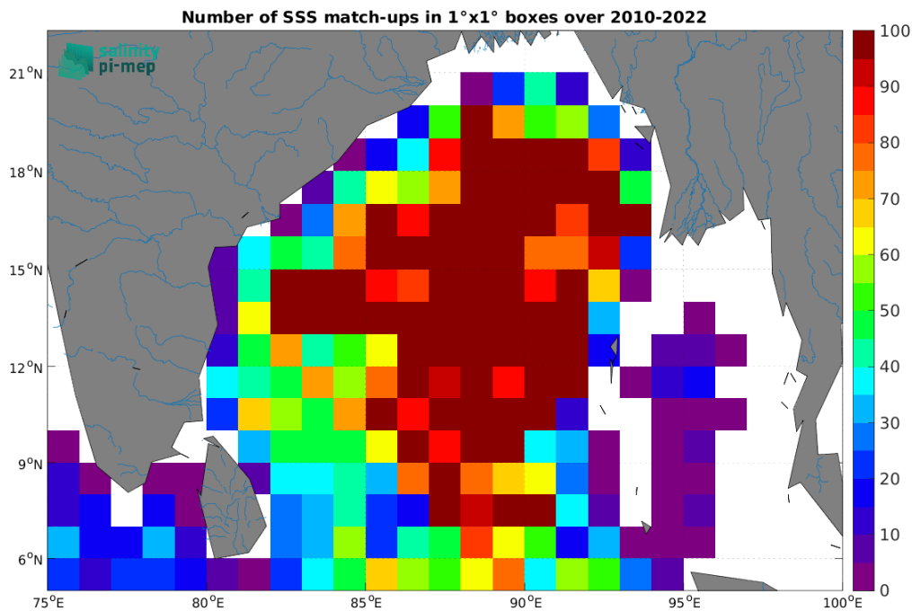
Figure 5: Number of SSS match-ups between Argo SSS and the CCI SSS L4 Merged-OI v4.41 - 7-day running (ESA) SSS product for the Ganga and Brahmaputra river plumes Pi-MEP region over 1^\circ \times 1^\circ boxes and for the full satellite product period.
