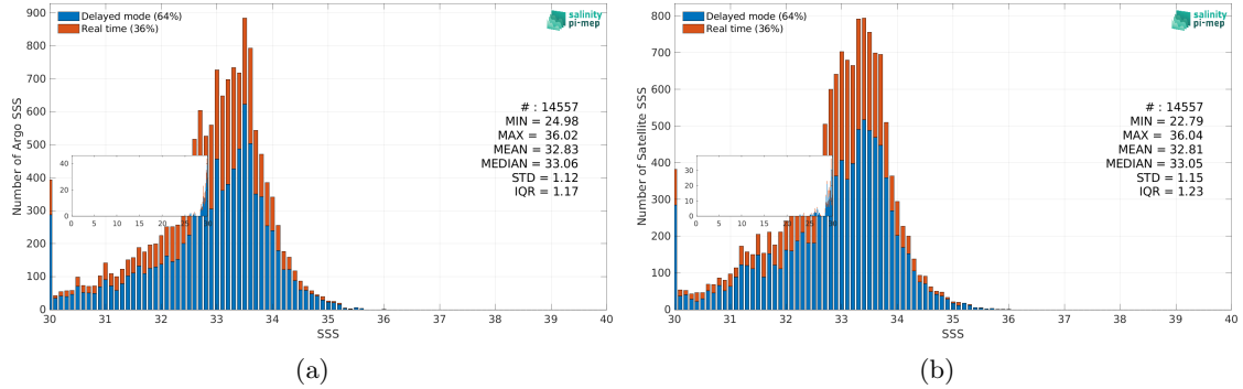
Figure 3: Histograms of SSS from Argo (a) and CCI SSS L4 Merged-OI v4.41 - 7-day running (ESA) (b) considering all match-up pairs per bins of 0.1 over the Ganga and Brahmaputra river plumes Pi-MEP region and for the full satellite product period.
