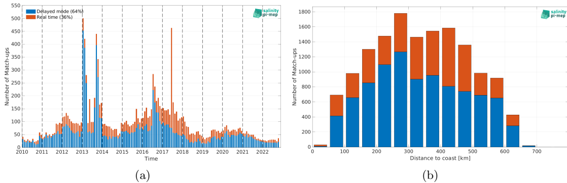
Figure 2: Number of match-ups between Argo and CCI SSS L4 Merged-OI v4.41 - 7-day running (ESA) SSS as a function of time (a) and as function of the distance to coast (b) over the Ganga and Brahmaputra river plumes Pi-MEP region and for the full satellite product period.
