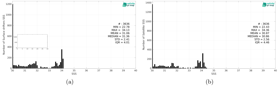
Figure 2: Histograms of SSS from Surface drifters (a) and CCI SSS L4 Merged-OI v4.4 - 7-day running (ESA) (b) considering all match-up pairs per bins of 0.1 over the Ganga and Brahmaputra river plumes Pi-MEP region and for the full satellite product period.
