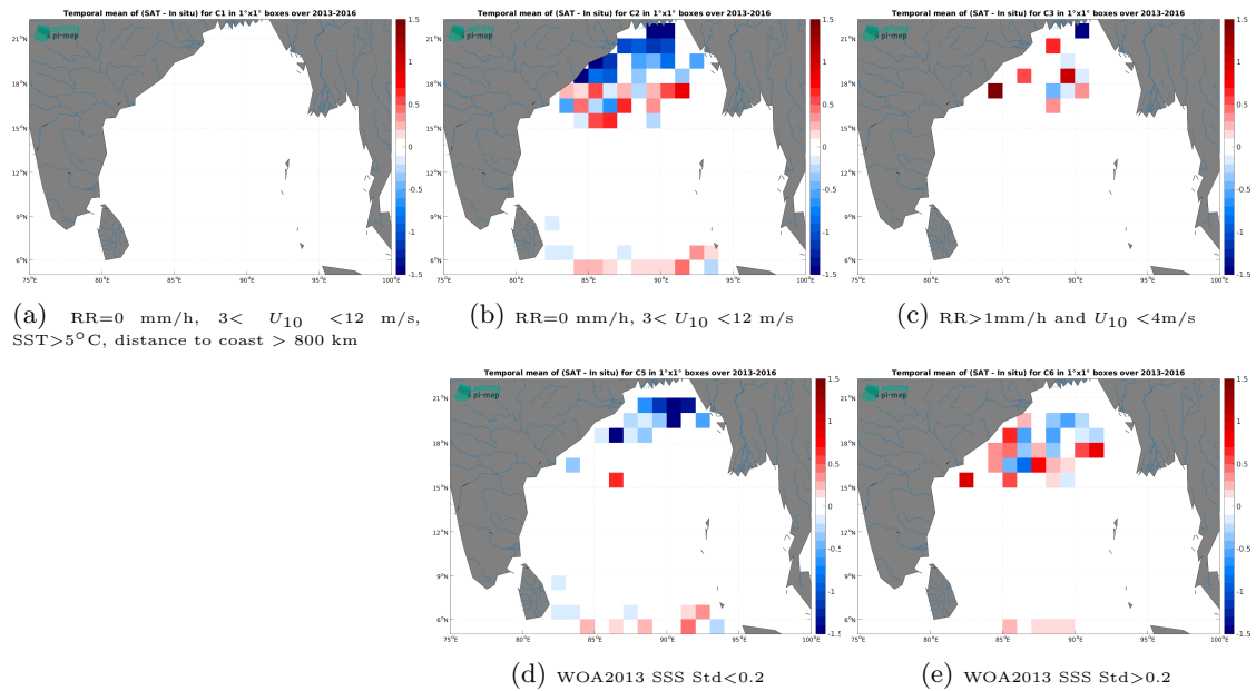
Figure 11: Temporal mean gridded over spatial boxes of size 1^\circ \times 1^\circ of \Delta SSS (CCI SSS L4 Merged-OI v4.4 - 7-day running (ESA) - Surface drifters) for 5 different subdatasets corresponding to:RR=0 mm/h, 3 < U_{10} < 12 m/s, SST >5^\circ\text{C} , distance to coast > 800 km (a), RR=0 mm/h, 3 < U_{10} < 12 m/s (b), RR >1 mm/h and U_{10} < 4 m/s (c), WOA2013 SSS Std <0.2 (d), WOA2013 SSS Std >0.2 (e).
