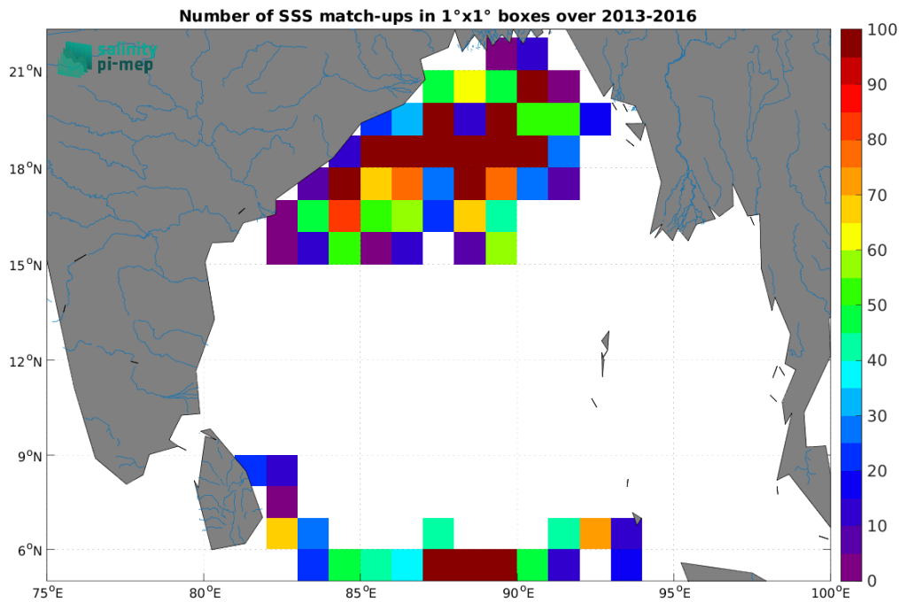
Figure 3: Number of SSS match-ups between Surface drifters SSS and the CCI SSS L4 Merged-OI v4.4 - 7-day running (ESA) SSS product for the Ganga and Brahmaputra river plumes Pi-MEP region over 1^\circ \times 1^\circ boxes and for the full satellite product period.
