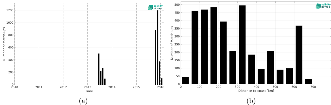
Figure 1: Number of match-ups between Surface drifters and CCI SSS L4 Merged-OI v4.4 - 7-day running (ESA) SSS as a function of time (a) and as function of the distance to coast (b) over the Ganga and Brahmaputra river plumes Pi-MEP region and for the full satellite product period.
