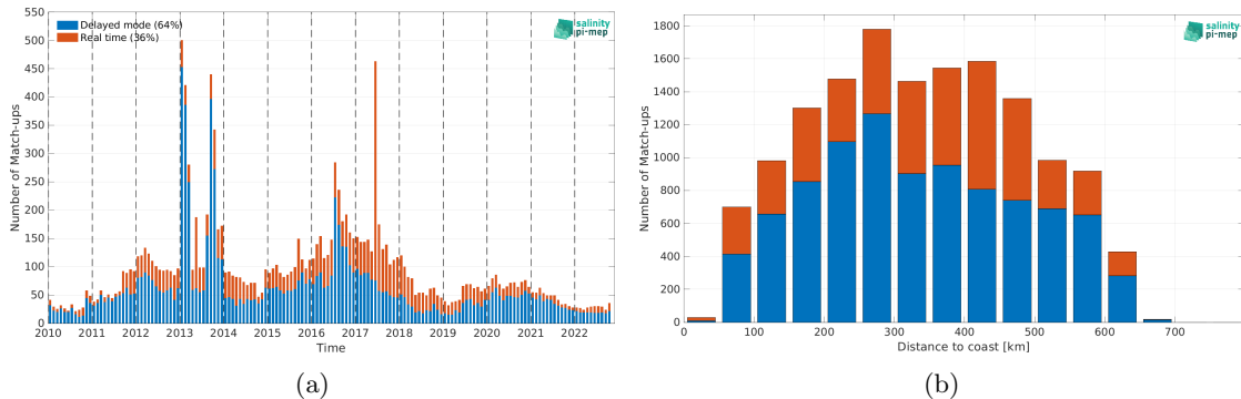
Figure 1: Number of match-ups between Argo and CCI SSS L4 Merged-OI v4.4 - 7-day running (ESA) SSS as a function of time (a) and as function of the distance to coast (b) over the Ganga and Brahmaputra river plumes Pi-MEP region and for the full satellite product period.
