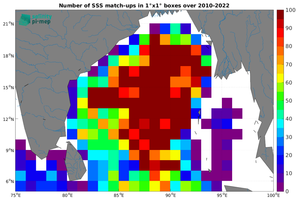
Figure 4: Number of SSS match-ups between Argo SSS and the CCI SSS L4 Merged-OI v4.4 - 7-day running (ESA) SSS product for the Ganga and Brahmaputra river plumes Pi-MEP region over 1^\circ \times 1^\circ boxes and for the full satellite product period.
