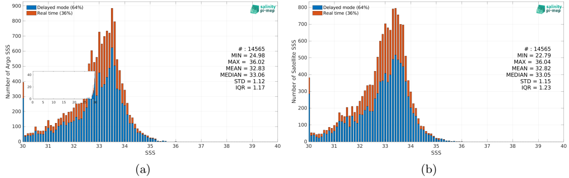
Figure 2: Histograms of SSS from Argo (a) and CCI SSS L4 Merged-OI v4.4 - 7-day running (ESA) (b) considering all match-up pairs per bins of 0.1 over the Ganga and Brahmaputra river plumes Pi-MEP region and for the full satellite product period.
