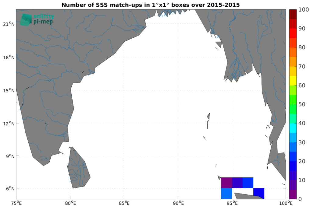
Figure 4: Number of SSS match-ups between TSG (SAMOS) SSS and the CCI SSS L4 Merged-OI v3.2 - 7-day running (ESA) SSS product for the Ganga and Brahmaputra river plumes Pi-MEP region over 1^{\circ} \times 1^{\circ} boxes and for the full satellite product period.
