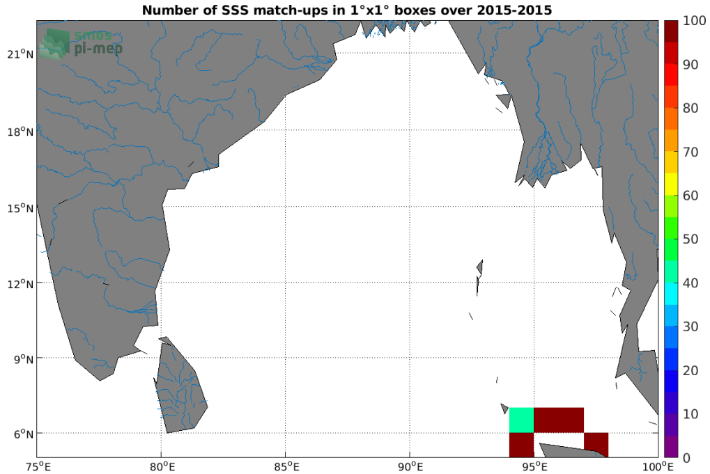
Figure 4: Number of SSS match-ups between TSG (SAMOS) SSS and the CCI SSS L4 Merged-OI v3.2 - 7-day running (ESA) SSS product for the Ganga and Brahmaputra river plumes Pi-MEP region over 1°x1° boxes and for the full satellite product period.
