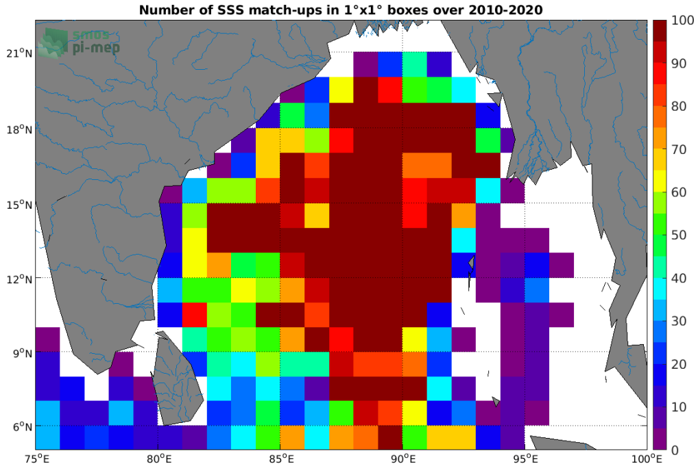
Figure 4: Number of SSS match-ups between Argo SSS and the CCI SSS L4 Merged-OI v3.2 - 7-day running (ESA) SSS product for the Ganga and Brahmaputra river plumes Pi-MEP region over 1°x1° boxes and for the full satellite product period.
