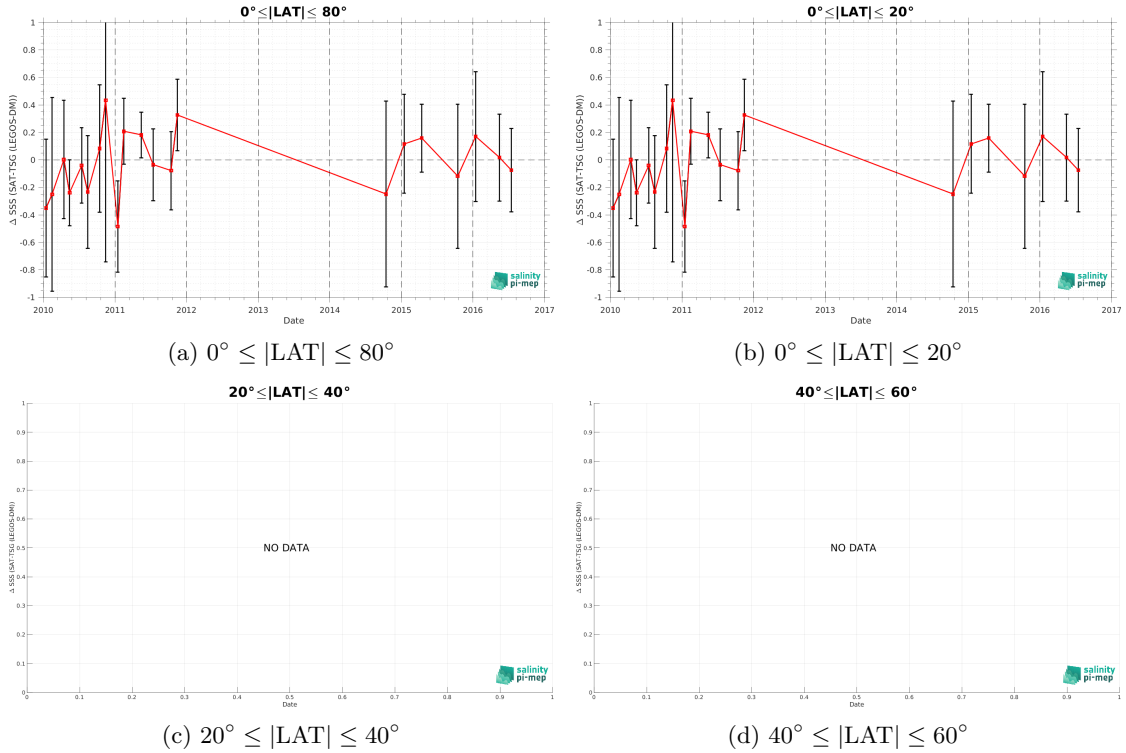
Figure 10: Monthly median (red curves) of \Delta SSS (Satellite - in situ ) between CCI SSS L4 Merged-OI v3.2 - 30-day running (ESA) and TSG (LEGOS-DM) SSS as function of time for all the collected Pi-MEP match-up pairs estimated over the Ganga and Brahmaputra river plumes Pi-MEP region and for the full satellite product period are shown for different latitude bands: (a) 80^\circ\text{S}-80^\circ\text{N} , (b) 20^\circ\text{S}-20^\circ\text{N} , (c) 40^\circ\text{S}-20^\circ\text{S} and 20^\circ\text{N}-40^\circ\text{N} and (d) 60^\circ\text{S}-40^\circ\text{S} and 40^\circ\text{N}-60^\circ\text{N} .
