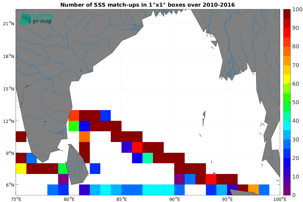
Figure 4: Number of SSS match-ups between TSG (LEGOS-DM) SSS and the CCI SSS L4 Merged-OI v3.2 - 30-day running (ESA) SSS product for the Ganga and Brahmaputra river plumes Pi-MEP region over 1^{\circ} \times 1^{\circ} boxes and for the full satellite product period.
