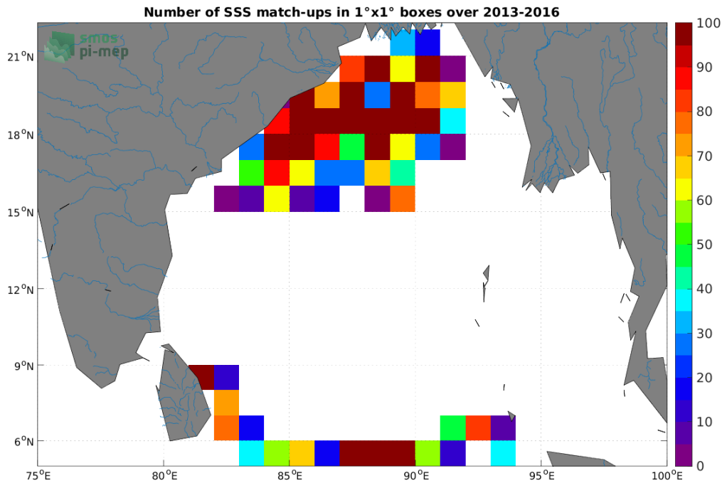
Figure 3: Number of SSS match-ups between Surface drifters SSS and the CCI SSS L4 Merged-OI v3.2 - 30-day running (ESA) SSS product for the Ganga and Brahmaputra river plumes Pi-MEP region over 1^{\circ} \times 1^{\circ} boxes and for the full satellite product period.
