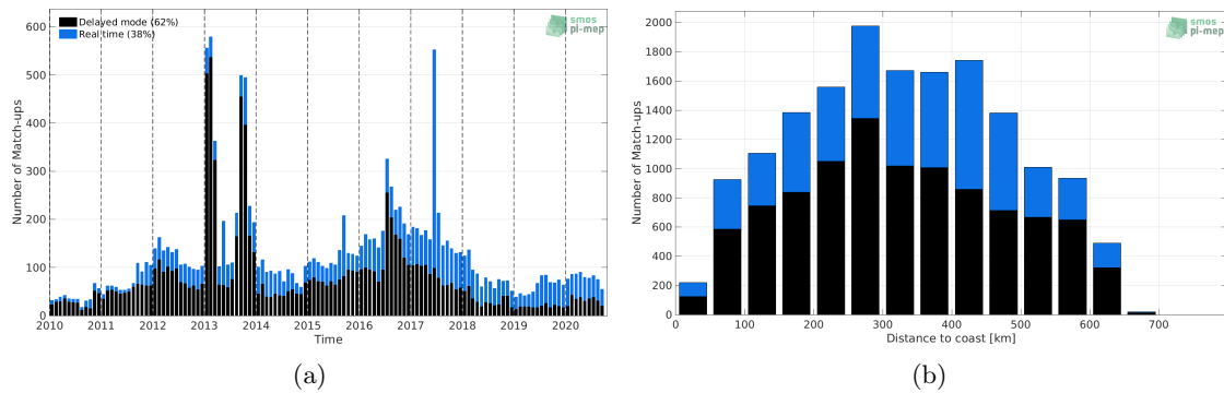
Figure 1: Number of match-ups between Argo and CCI SSS L4 Merged-OI v3.2 - 30-day running (ESA) SSS as a function of time (a) and as function of the distance to coast (b) over the Ganga and Brahmaputra river plumes Pi-MEP region and for the full satellite product period.
