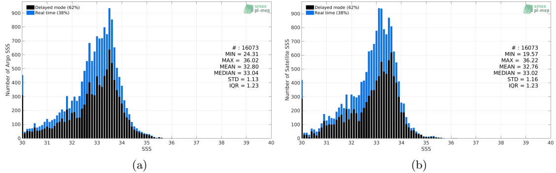
Figure 2: Histograms of SSS from Argo (a) and CCI SSS L4 Merged-OI v3.2 - 30-day running (ESA) (b) considering all match-up pairs per bins of 0.1 over the Ganga and Brahmaputra river plumes Pi-MEP region and for the full satellite product period.
