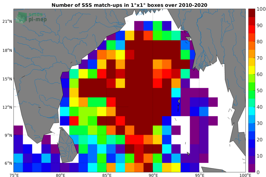
Figure 4: Number of SSS match-ups between Argo SSS and the CCI SSS L4 Merged-OI v3.2 - 30-day running (ESA) SSS product for the Ganga and Brahmaputra river plumes Pi-MEP region over 1^{\circ} \times 1^{\circ} boxes and for the full satellite product period.
