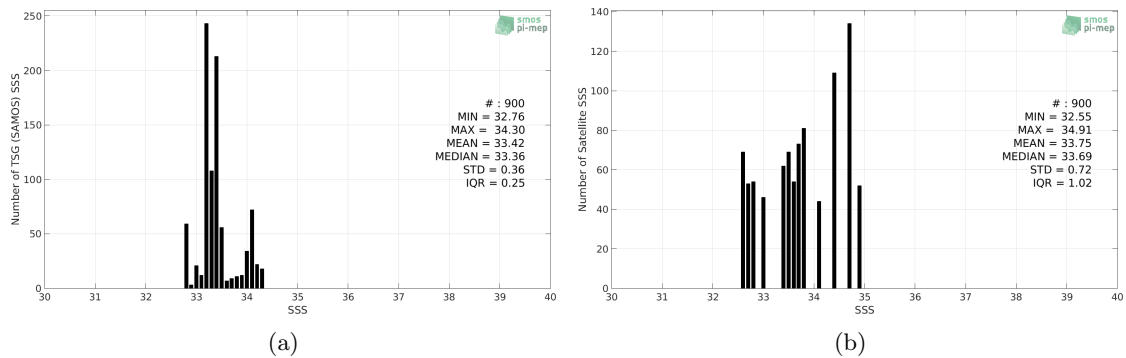
Figure 2: Histograms of SSS from TSG (SAMOS) (a) and CCI SSS L4 Merged-OI v2.31 - 7-day running (ESA) (b) considering all match-up pairs per bins of 0.1 over the Ganga and Brahmaputra river plumes Pi-MEP region and for the full satellite product period.
