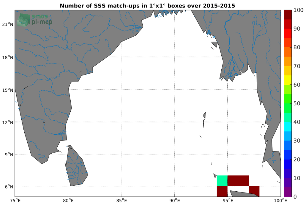
Figure 4: Number of SSS match-ups between TSG (SAMOS) SSS and the CCI SSS L4 Merged-OI v2.31 - 7-day running (ESA) SSS product for the Ganga and Brahmaputra river plumes Pi-MEP region over 1°x1° boxes and for the full satellite product period.
