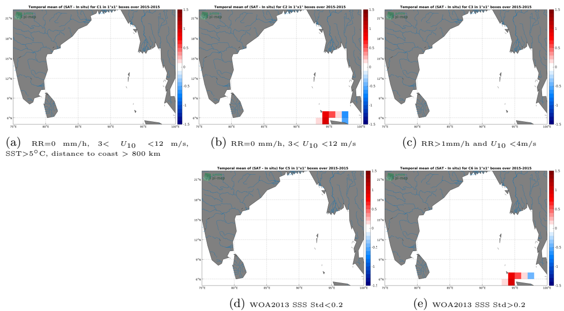
Figure 12: Temporal mean gridded over spatial boxes of size 1°x1° of \Delta SSS (CCI SSS L4 Merged-OI v2.31 - 7-day running (ESA) - TSG (SAMOS)) for 5 different subdatasets corresponding to:RR=0 mm/h, 3 < U_{10} < 12 m/s, SST>5°C, distance to coast > 800 km (a), RR=0 mm/h, 3 < U_{10} < 12 m/s (b), RR>1mm/h and U_{10} < 4 m/s (c), WOA2013 SSS Std<0.2 (d), WOA2013 SSS Std>0.2 (e).
