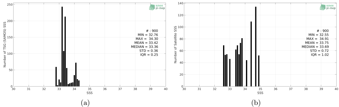
Figure 2: Histograms of SSS from TSG (SAMOS) (a) and CCI L4 Merged-OI v2.31 - 7-day running (ESA) (b) considering all match-up pairs per bins of 0.1 over the Ganga and Brahmaputra river plumes Pi-MEP region and for the full satellite product period.
