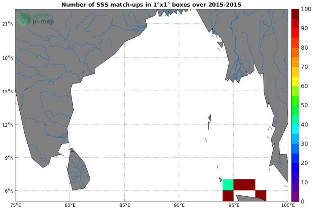
Figure 4: Number of SSS match-ups between TSG (SAMOS) SSS and the CCI L4 Merged-OI v2.31 - 7-day running (ESA) SSS product for the Ganga and Brahmaputra river plumes Pi-MEP region over 1°x1° boxes and for the full satellite product period.
