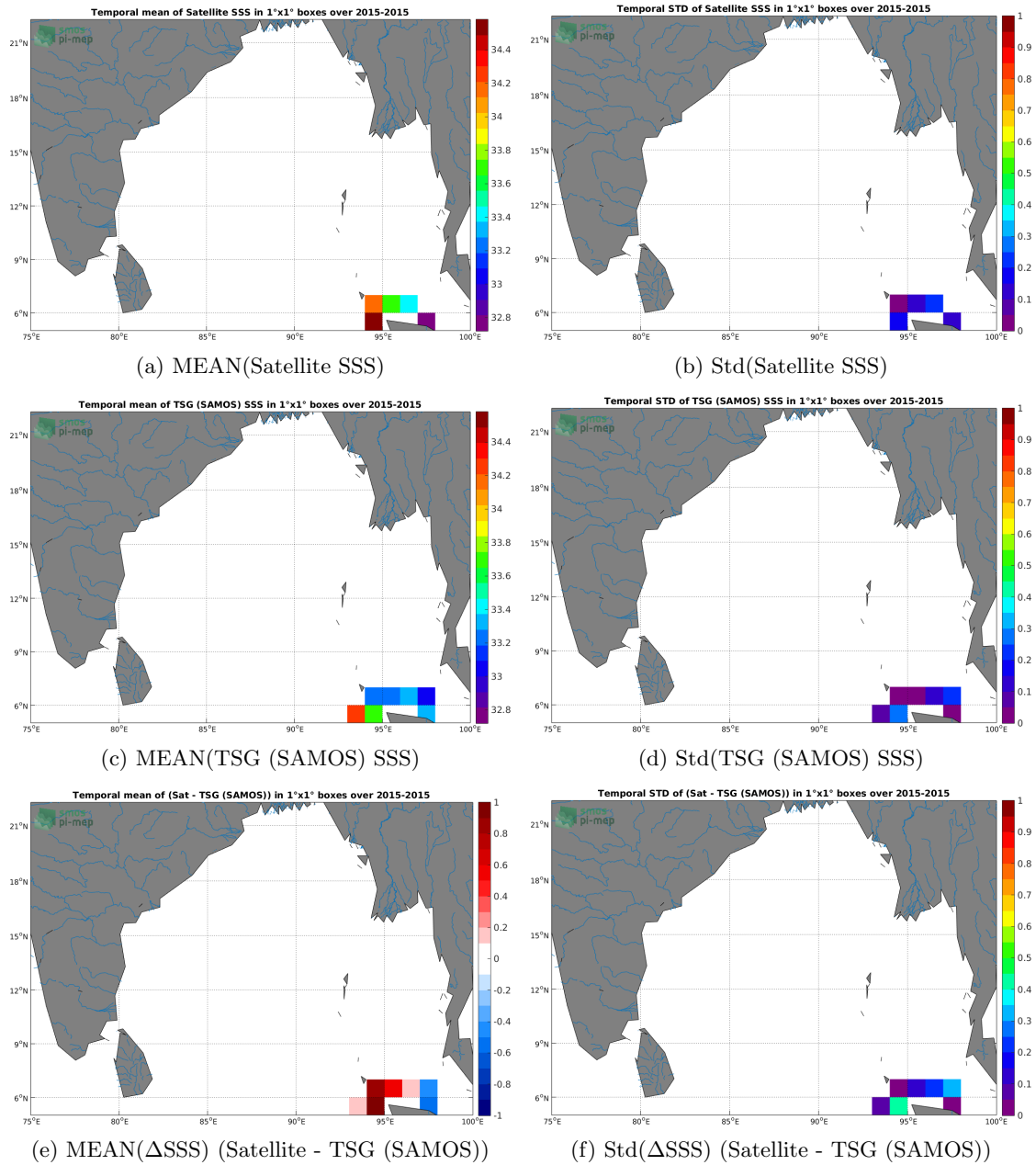
Figure 6: Temporal mean (left) and Std (right) of SSS from CCI L4 Merged-OI v2.31 - 7-day running (ESA) (top), TSG (SAMOS) (middle), and of \Delta SSS (Satellite - TSG (SAMOS)). Only match-up pairs are used to generate these maps.
