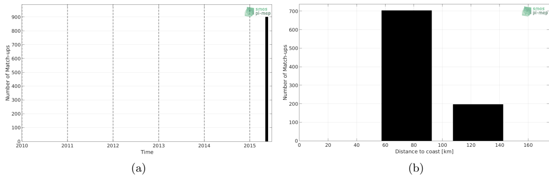
Figure 1: Number of match-ups between TSG (SAMOS) and CCI L4 Merged-OI v2.31 - 7-day running (ESA) SSS as a function of time (a) and as function of the distance to coast (b) over the Ganga and Brahmaputra river plumes Pi-MEP region and for the full satellite product period.
