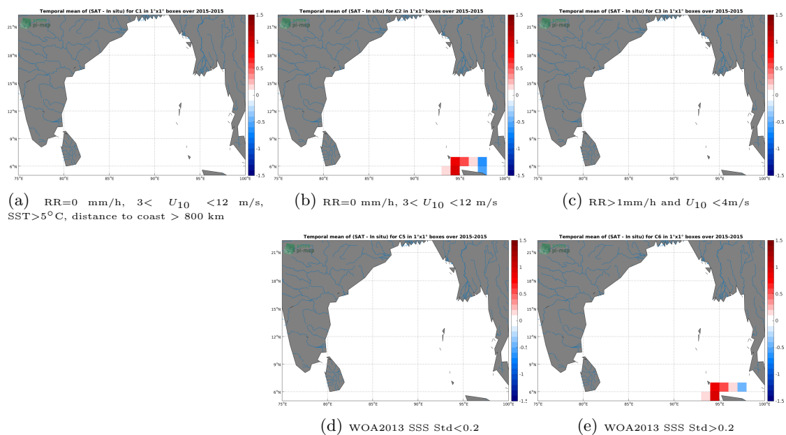
Figure 12: Temporal mean gridded over spatial boxes of size 1^\circ \times 1^\circ of \Delta SSS (CCI L4 Merged-OI v2.31 - 7-day running (ESA) - TSG (SAMOS)) for 5 different subdatasets corresponding to:RR=0 mm/h, 3 < U_{10} < 12 m/s, SST >5^\circ\text{C} , distance to coast > 800 km (a), RR=0 mm/h, 3 < U_{10} < 12 m/s (b), RR >1 mm/h and U_{10} < 4 m/s (c), WOA2013 SSS Std <0.2 (d), WOA2013 SSS Std >0.2 (e).
