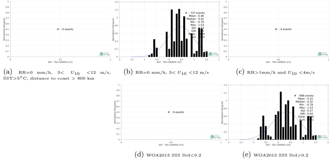
Figure 13: Normalized histogram of \Delta SSS (CCI L4 Merged-OI v2.31 - 7-day running (ESA) - TSG (SAMOS)) for 5 different subdatasets corresponding to: RR=0 mm/h, 3 < U_{10} < 12 m/s, SST>5°C, distance to coast > 800 km (a), RR=0 mm/h, 3 < U_{10} < 12 m/s (b), RR>1mm/h and U_{10} < 4 m/s (c), WOA2013 SSS Std<0.2 (d), WOA2013 SSS Std>0.2 (e).
