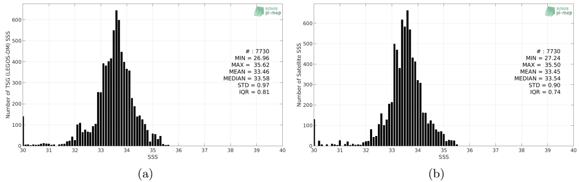
Figure 2: Histograms of SSS from TSG (LEGOS-DM) (a) and CCI SSS L4 Merged-OI v2.31 - 7-day running (ESA) (b) considering all match-up pairs per bins of 0.1 over the Ganga and Brahmaputra river plumes Pi-MEP region and for the full satellite product period.
