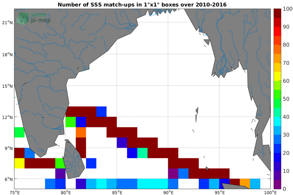
Figure 4: Number of SSS match-ups between TSG (LEGOS-DM) SSS and the CCI SSS L4 Merged-OI v2.31 - 7-day running (ESA) SSS product for the Ganga and Brahmaputra river plumes Pi-MEP region over 1^\circ \times 1^\circ boxes and for the full satellite product period.
