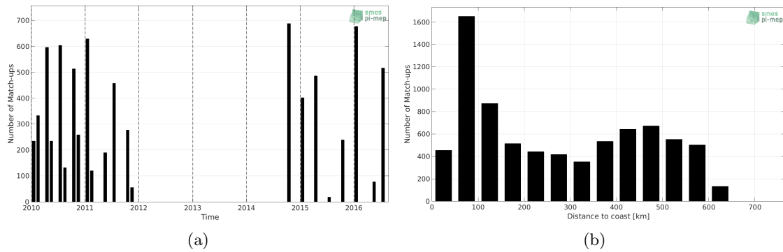
Figure 1: Number of match-ups between TSG (LEGOS-DM) and CCI SSS L4 Merged-OI v2.31 - 7-day running (ESA) SSS as a function of time (a) and as function of the distance to coast (b) over the Ganga and Brahmaputra river plumes Pi-MEP region and for the full satellite product period.
