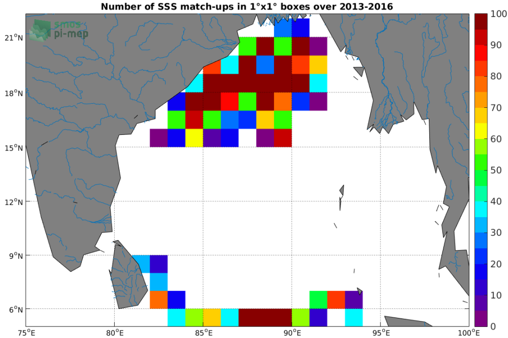
Figure 3: Number of SSS match-ups between Surface drifters SSS and the CCI SSS L4 Merged-OI v2.31 - 7-day running (ESA) SSS product for the Ganga and Brahmaputra river plumes Pi-MEP region over 1°x1° boxes and for the full satellite product period.
