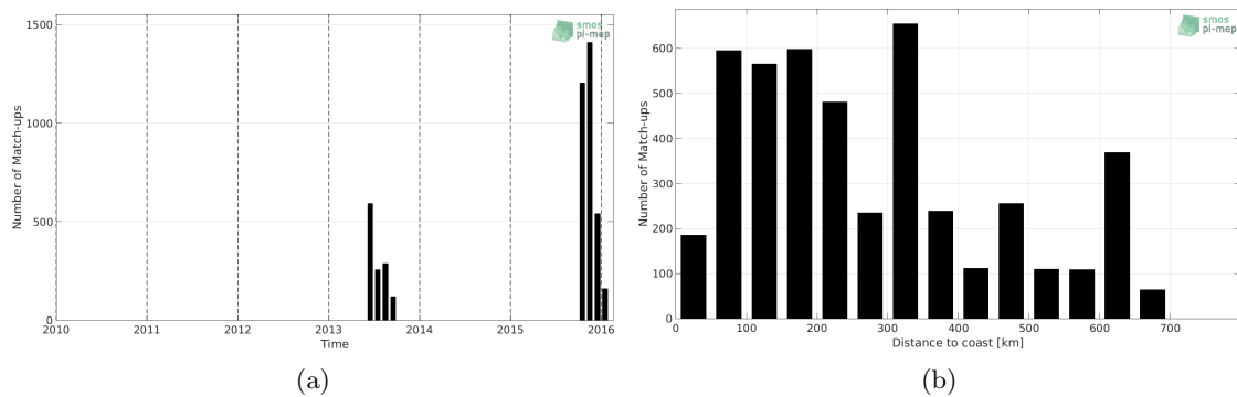
Figure 1: Number of match-ups between Surface drifters and CCI SSS L4 Merged-OI v2.31 - 7-day running (ESA) SSS as a function of time (a) and as function of the distance to coast (b) over the Ganga and Brahmaputra river plumes Pi-MEP region and for the full satellite product period.
