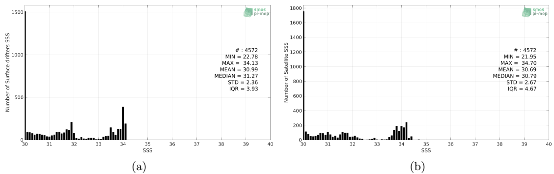
Figure 2: Histograms of SSS from Surface drifters (a) and CCI SSS L4 Merged-OI v2.31 - 7-day running (ESA) (b) considering all match-up pairs per bins of 0.1 over the Ganga and Brahmaputra river plumes Pi-MEP region and for the full satellite product period.
