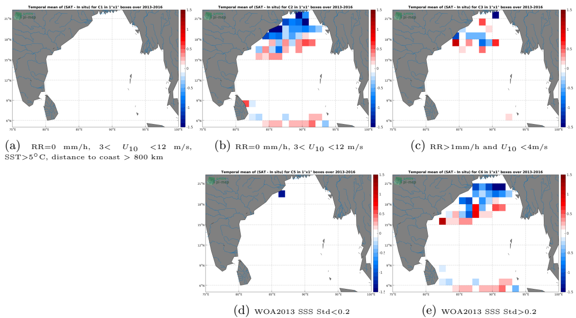
Figure 11: Temporal mean gridded over spatial boxes of size 1°x1° of \Delta SSS (CCI SSS L4 Merged-OI v2.31 - 7-day running (ESA) - Surface drifters) for 5 different subdatasets corresponding to:RR=0 mm/h, 3 < U_{10} < 12 m/s, SST>5°C, distance to coast > 800 km (a), RR=0 mm/h, 3 < U_{10} < 12 m/s (b), RR>1mm/h and U_{10} < 4 m/s (c), WOA2013 SSS Std<0.2 (d), WOA2013 SSS Std>0.2 (e).
