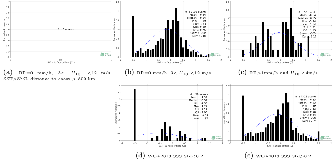
Figure 12: Normalized histogram of \Delta SSS (CCI SSS L4 Merged-OI v2.31 - 7-day running (ESA) - Surface drifters) for 5 different subdatasets corresponding to: RR=0 mm/h, 3 < U_{10} < 12 m/s, SST>5°C, distance to coast > 800 km (a), RR=0 mm/h, 3 < U_{10} < 12 m/s (b), RR>1mm/h and U_{10} < 4 m/s (c), WOA2013 SSS Std<0.2 (d), WOA2013 SSS Std>0.2 (e).
