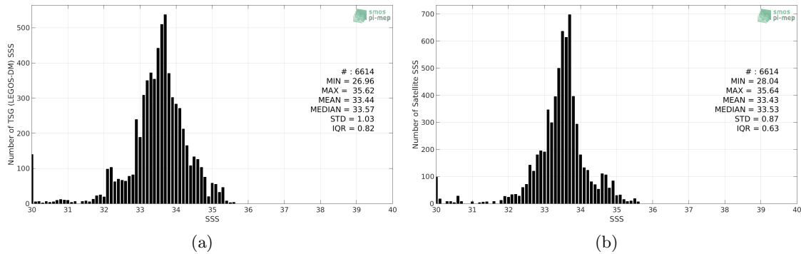
Figure 2: Histograms of SSS from TSG (LEGOS-DM) (a) and CCI L4 Merged-OI v2.31 - 30-day running (ESA) (b) considering all match-up pairs per bins of 0.1 over the Ganga and Brahmaputra river plumes Pi-MEP region and for the full satellite product period.
