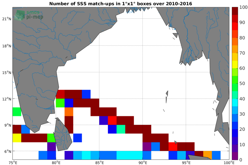
Figure 4: Number of SSS match-ups between TSG (LEGOS-DM) SSS and the CCI L4 Merged-OI v2.31 - 30-day running (ESA) SSS product for the Ganga and Brahmaputra river plumes Pi-MEP region over 1^\circ \times 1^\circ boxes and for the full satellite product period.
