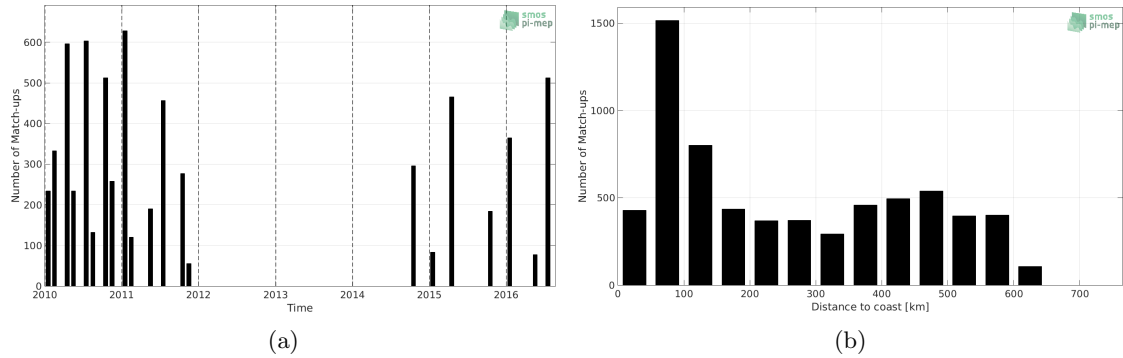
Figure 1: Number of match-ups between TSG (LEGOS-DM) and CCI L4 Merged-OI v2.31 - 30-day running (ESA) SSS as a function of time (a) and as function of the distance to coast (b) over the Ganga and Brahmaputra river plumes Pi-MEP region and for the full satellite product period.
